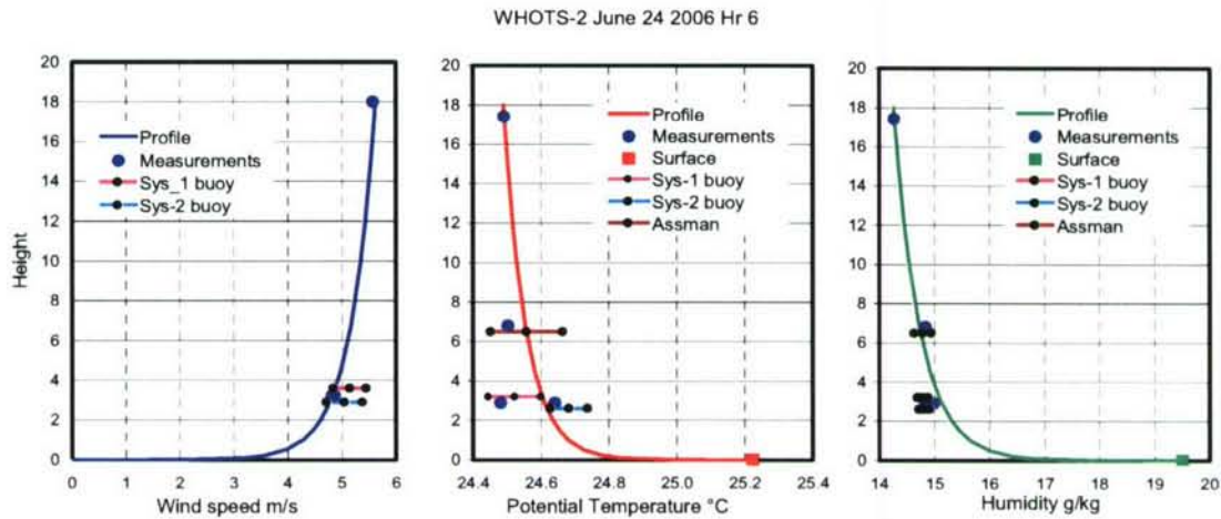
Figure 9. Example of profiles used for height adjustment of the various measurements during I/C1. The ship's anemometer was at 18m on the foremast, and the temperature/humidity (T/RH) sensor at 17.4 m. Temperature and humidity were measured with an Assman psychrometer through a forward chock at 6.8 m height. The ship was standing about 0.25 nm downwind of the WHOI buoy, which had two wind sensors at 3.22 m above the sea surface and two T/RH sensors at 2.88 m. The ship and buoy data points are hourly averages; the Assman values are spot readings. The profiles were constructed from flux/gradient parameters calculated using version 3.0 of the COARE bulk flux algorithm. A linear height scale is used to illustrate more clearly the characteristics of near-surface profiles over the ocean. Because the sea is very "smooth" compared with land surfaces (typically, z_0 over grassland is 0.01 m), most of the sea-air difference occurs in the lowest 1-2 meters.
