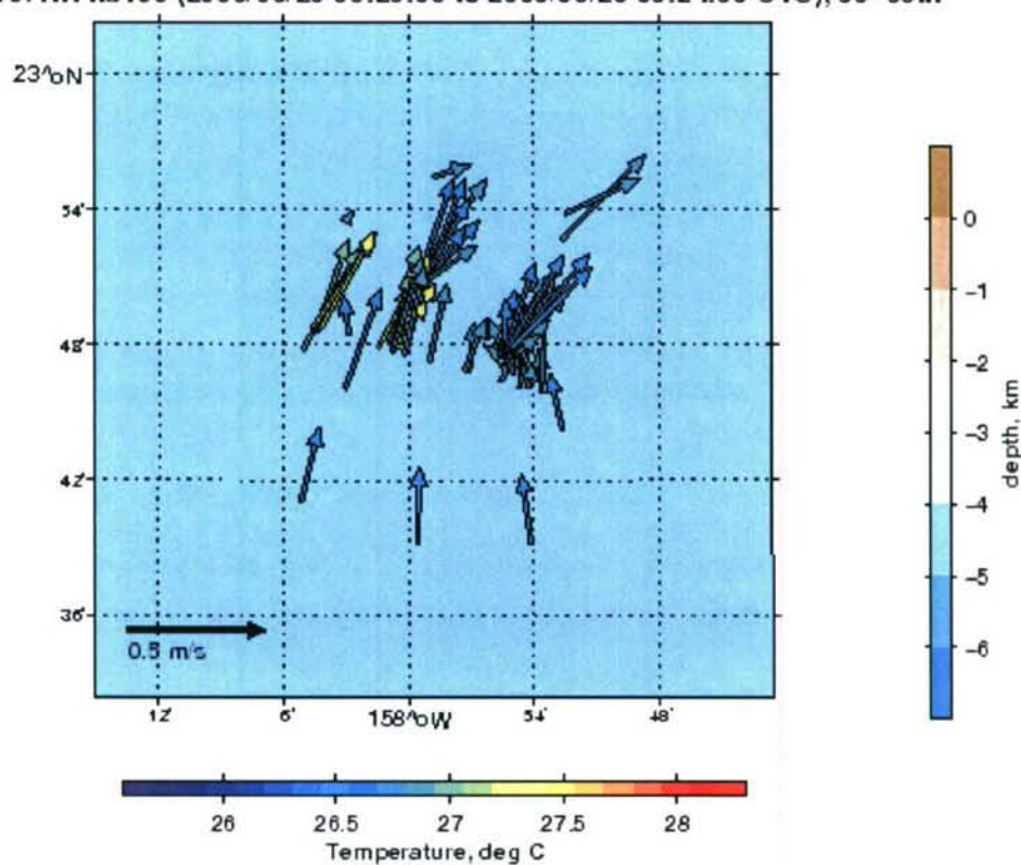
Figure 17. Current vectors for the 35-50 m layer measured by the R/V Revelle while working around the WHOTS site during the dates indicated.
