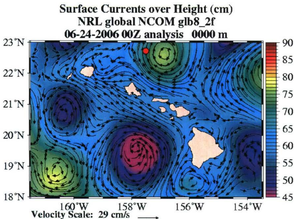
Figure 18. Hawaii region sea level and surface current analysis from the Navy NCOM system for 6/24/06. Note the anticyclonic eddy feature to the east of Station ALOHA (indicated by red dot.)
