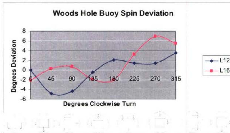
Figure 3. Woods Hole buoy spin deviation results.
