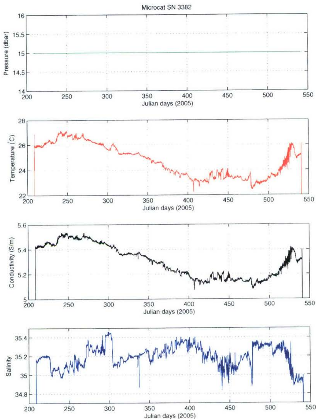
Figure A1: Preliminary Temperature, Conductivity and Salinity from SBE 37 SN3382 Microcat instrument deployed at 15m during the 2005 WHOTS-2 cruise and recovered during the 2006 WHOTS-3 cruise. Nominal pressure is also included to calculate salinity where pressure data was not available.
