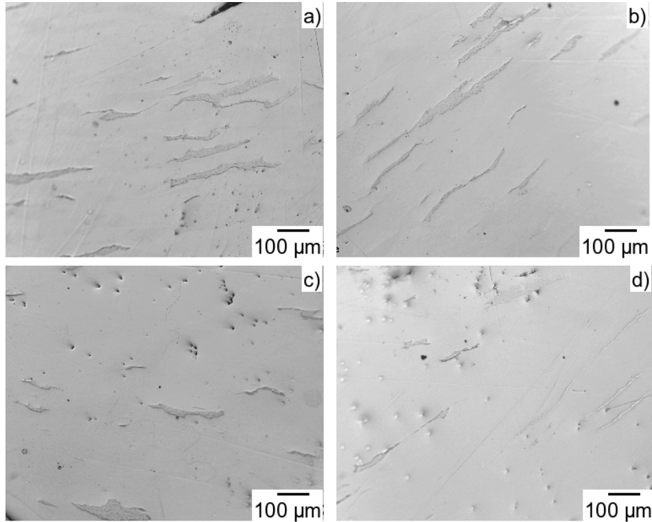
Fig. 23 Optical micrographs of compacts processed by ECAE with 175 MPa of back pressure at temperatures of: (a) 100 °C; (b) 200 °C; (c) 300 °C; (d) 400 °C
