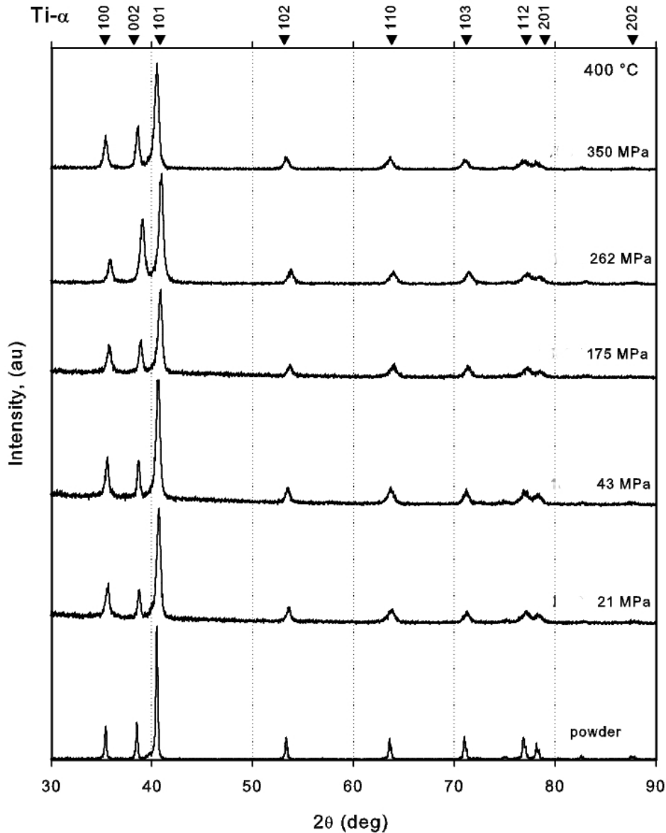
Fig. 37 XRD measurements of Ti64 powder and billets processed by ECAE at 400°C.
