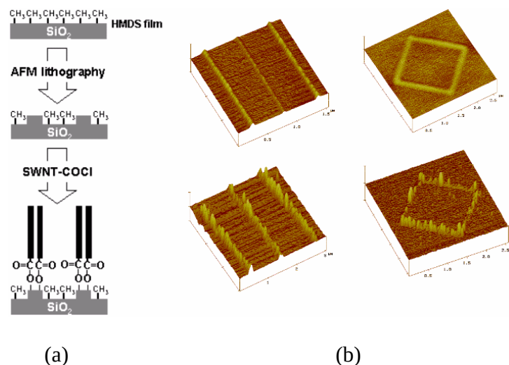
Figure 4 (a) Schematic for selective attachments of SWNTs on prepatterned surfaces, representative tapping mode AFM images of patterned HAMD SAM (b, top) before and (b, bottom) after reaction with SWNTs.
