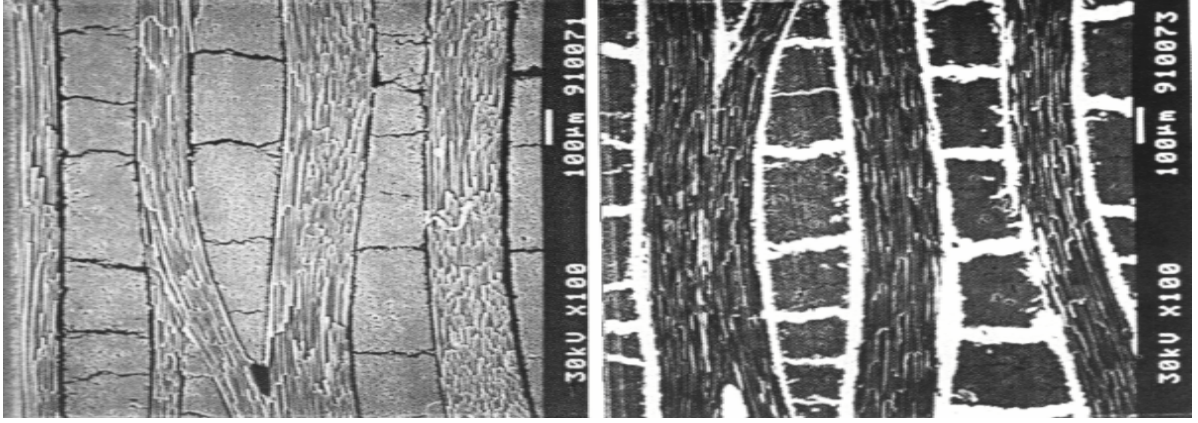
Fig. 2. Left handside micrograph of after pyrolysis at 900°C and right handside after siliconising process.
