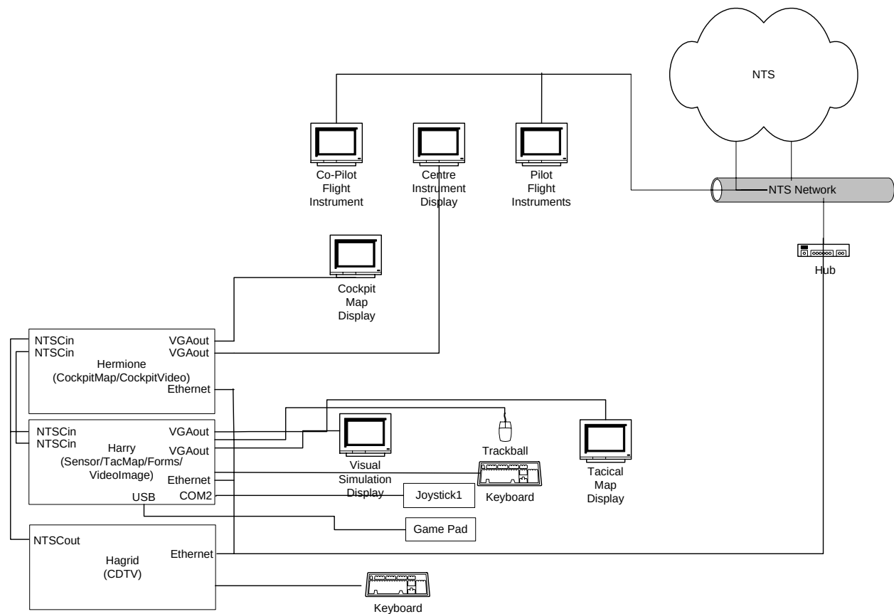
Figure 1-1 Stage 2 (Experiment #3) TAMSS-ERSTA System Configuration
