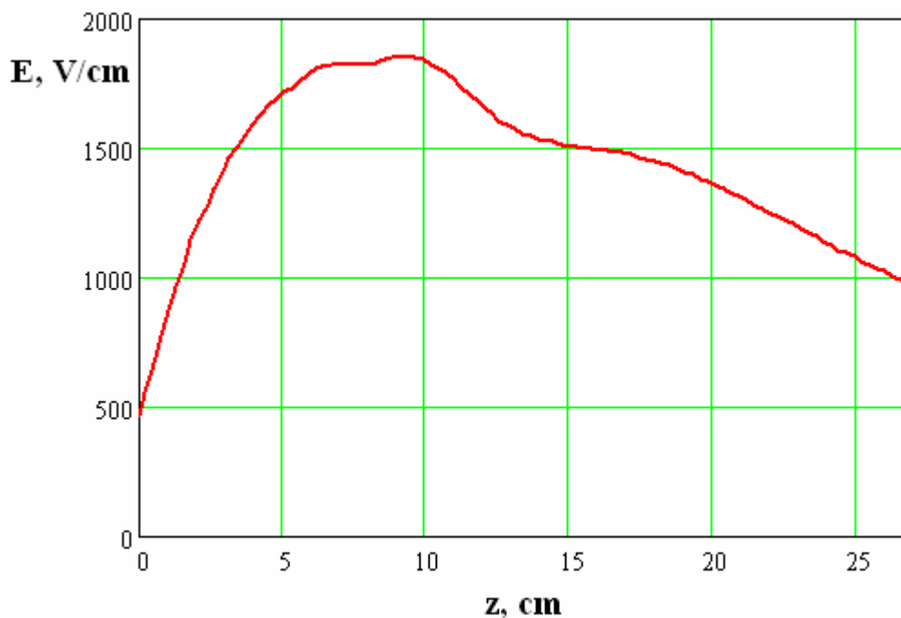
Fig.8.2.5. Results of MW electric field calculation in the scheme with the axicon lens.
