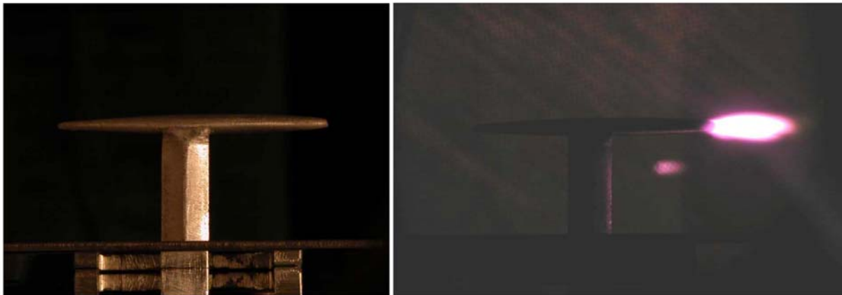
Fig.6.1.2. Appearance of deeply undercritical MW discharge initiated by a thin sharpened vibrator in a high-speed flow.
