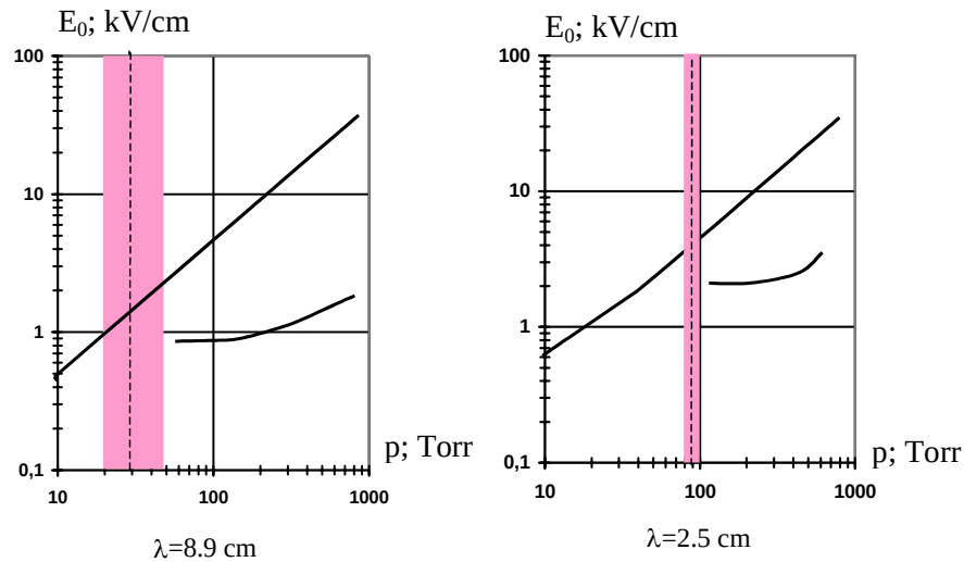
Fig.5.4.2. Existence areas of MW discharge different types in quasi-optical EM beams at \lambda = 8.9 \text{ cm} (to the left) and \lambda = 2.5 \text{ cm} (to the right)
