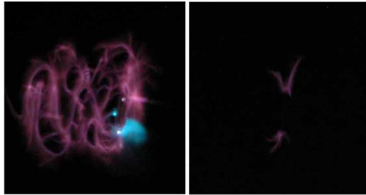
Fig.5.4.1. Photos of typical microwave discharges initiated by a vibrator with 2a = 1 \text{ mm} 2L = 7 \text{ mm} ; a left photo corresponds to the undercritical discharge; the right photo- to the deeply undercritical discharge
