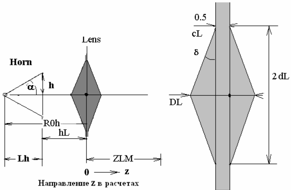
Fig. 8.2.4. Scheme with a conic lens (axicon) and its geometric shape.
