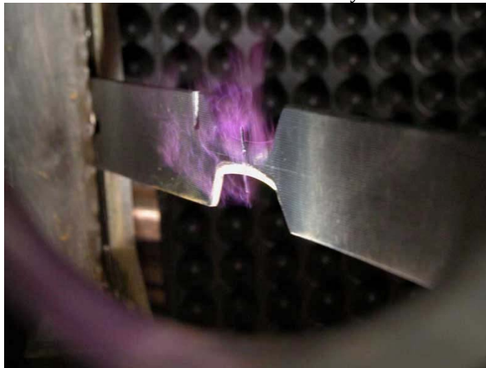
Fig.5.9.5.4. Appearance of the undercritical MW discharge in the high-speed air flow at v_{fl} \approx 500 m/s
