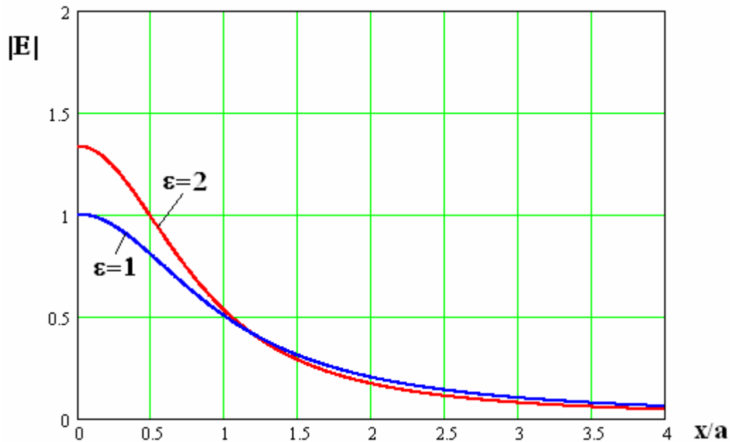
Fig.9.5.1. Distribution of the electric field module of the charge located above a flat dielectric surface with permittivity \varepsilon = 1 (dark blue line) and \varepsilon = 2 (red line) at q = 1 , a = 1 , z = 0 .
