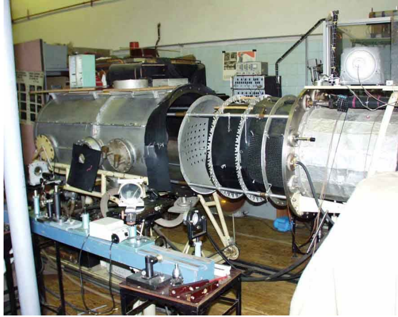
Fig.3.1.3. The appearance of the setup with \lambda = 8.9 \text{ cm} and open working chamber
