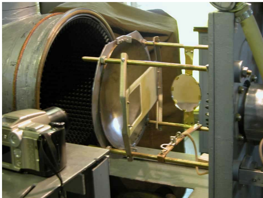
Fig.7.2.1.5 Appearance of the chamber's working area in experiments on investigations of surface transversal MW discharge with application of a flat mirror
