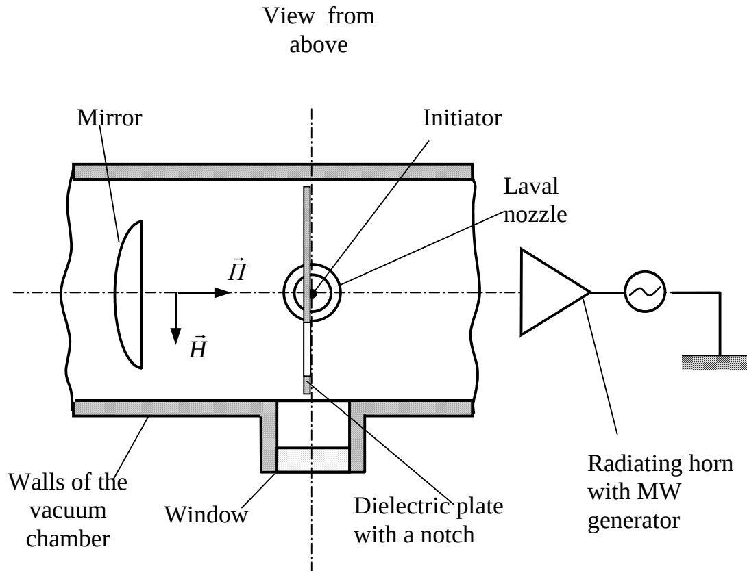
Fig.7.2.2.3. Experimental scheme on investigations of surface transversal MW discharge in the plane strictly perpendicular to the vector \Pi
