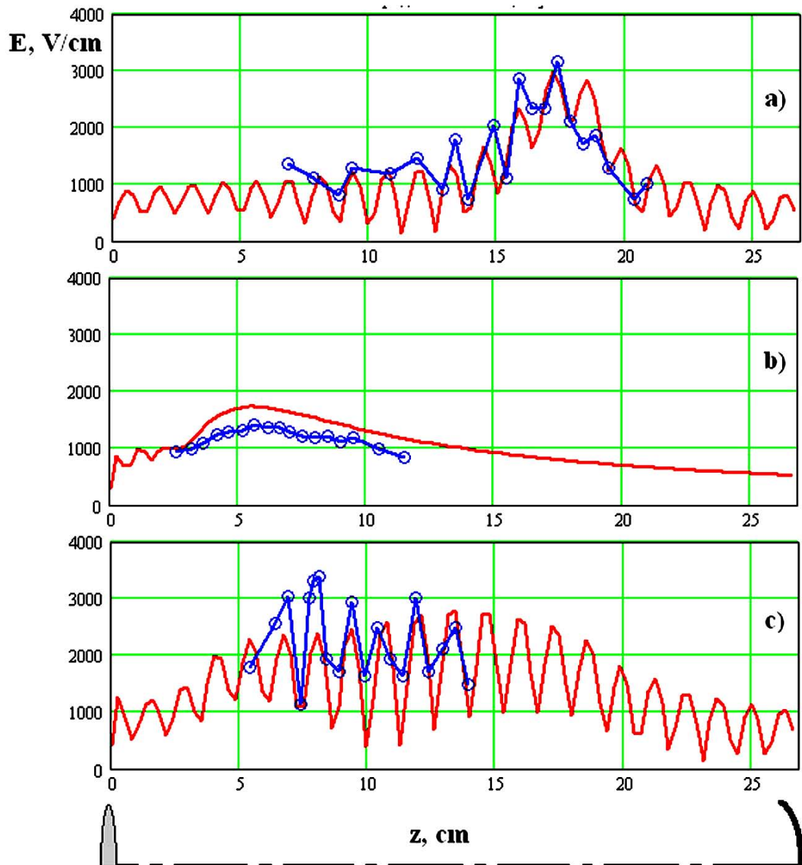
Fig.8.2.3. Comparison of the electric field amplitude calculated distributions along the axis z of experimental chamber: scheme I (a) – horn + mirror, scheme II (b) – horn + lens, and scheme III (c) – horn + lens + mirror. Calculated values of electric fields correspond to radiation power of 50 kW.
