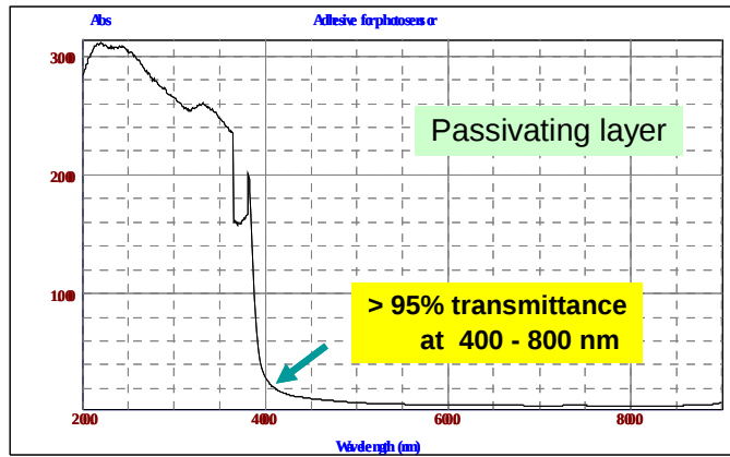
Figure 7. Optical property of the passivation layer.
