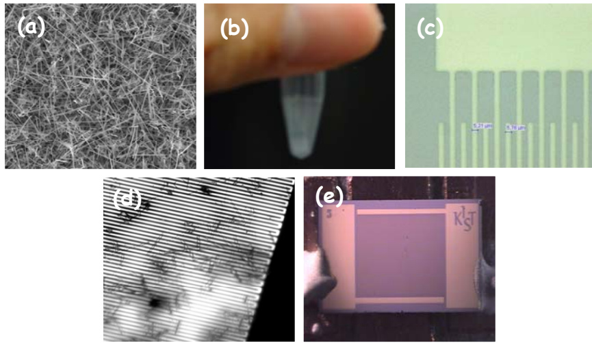
Figure 6. Fabrication procedure of nanowire-based photo-detector.
