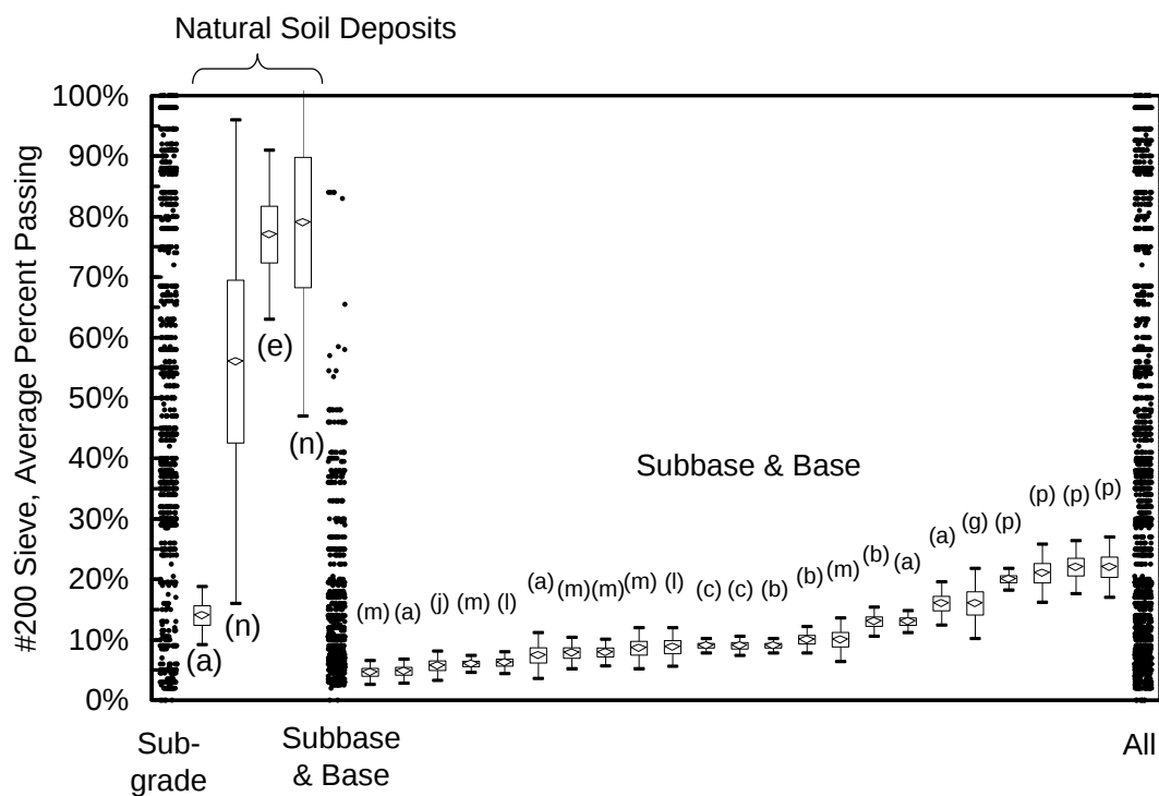
Figure C14. Comparison of database records and literature reports of average percent passing the #200 sieve.
