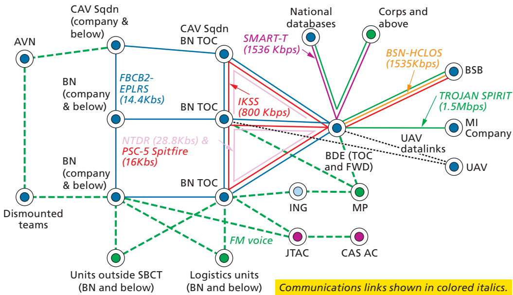
Figure 3.2 3/2 SBCT Communications Network
