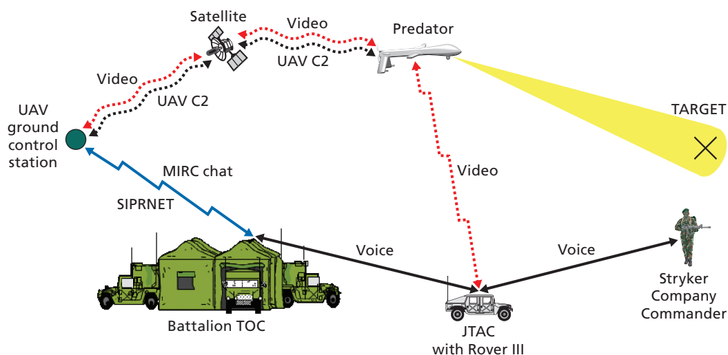
Figure 3.5 Predator Control Using Rover III and SIPRNET MIRC
