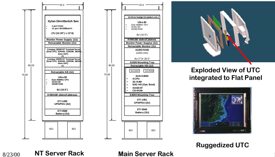
Figure 12. Breakdown of Windows NT and Main Server Racks in Q-70 Architecture 63
