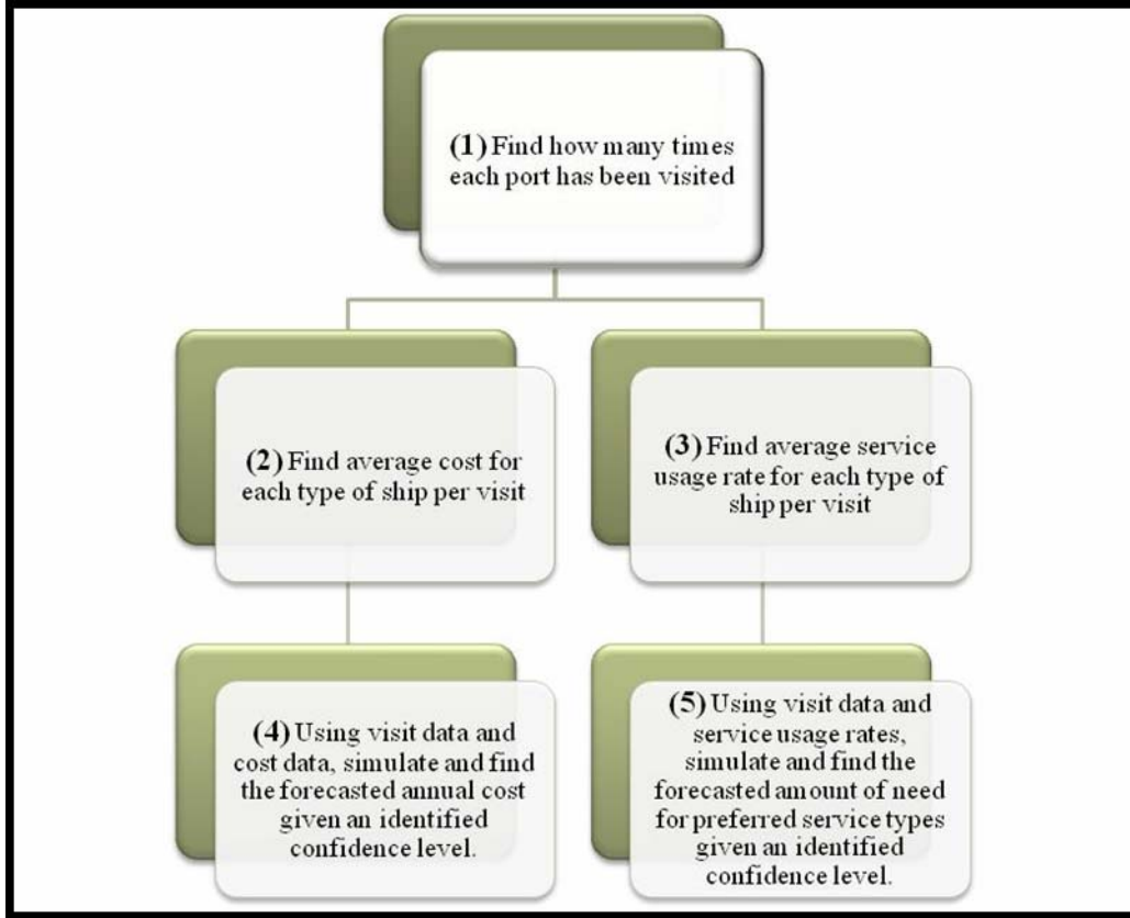
Figure 9. Modeling Algorithm
