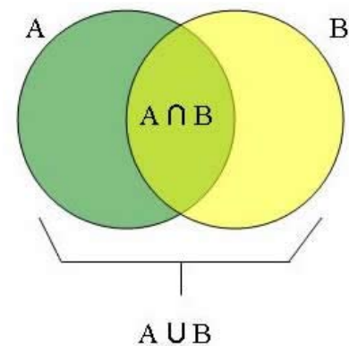
Figure 1: Knowledge held in common as a proportion of all knowledge: A \cap B / A \cup B .
