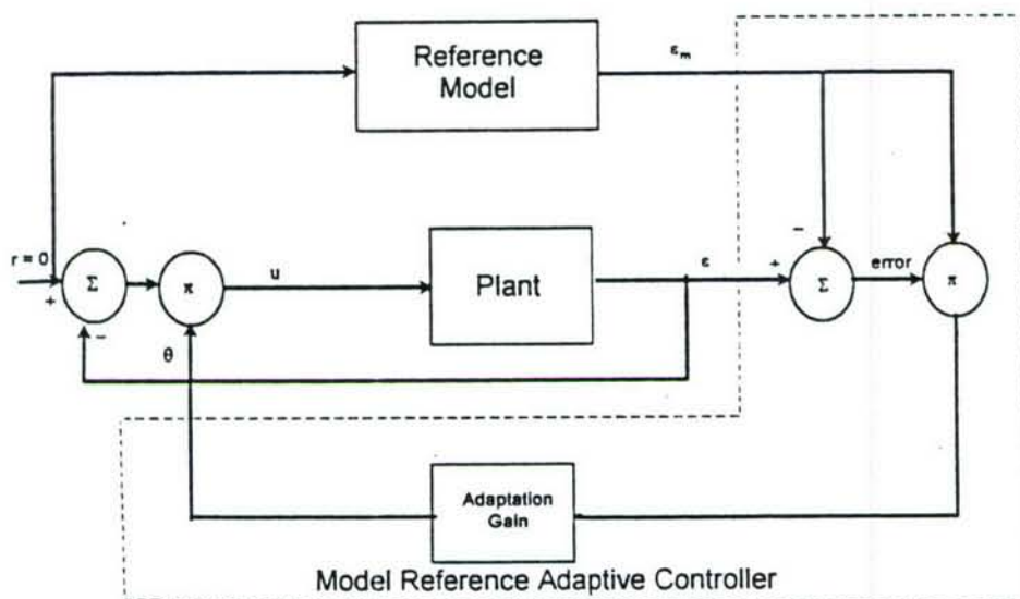
Figure 35 MRAC Block Diagram
