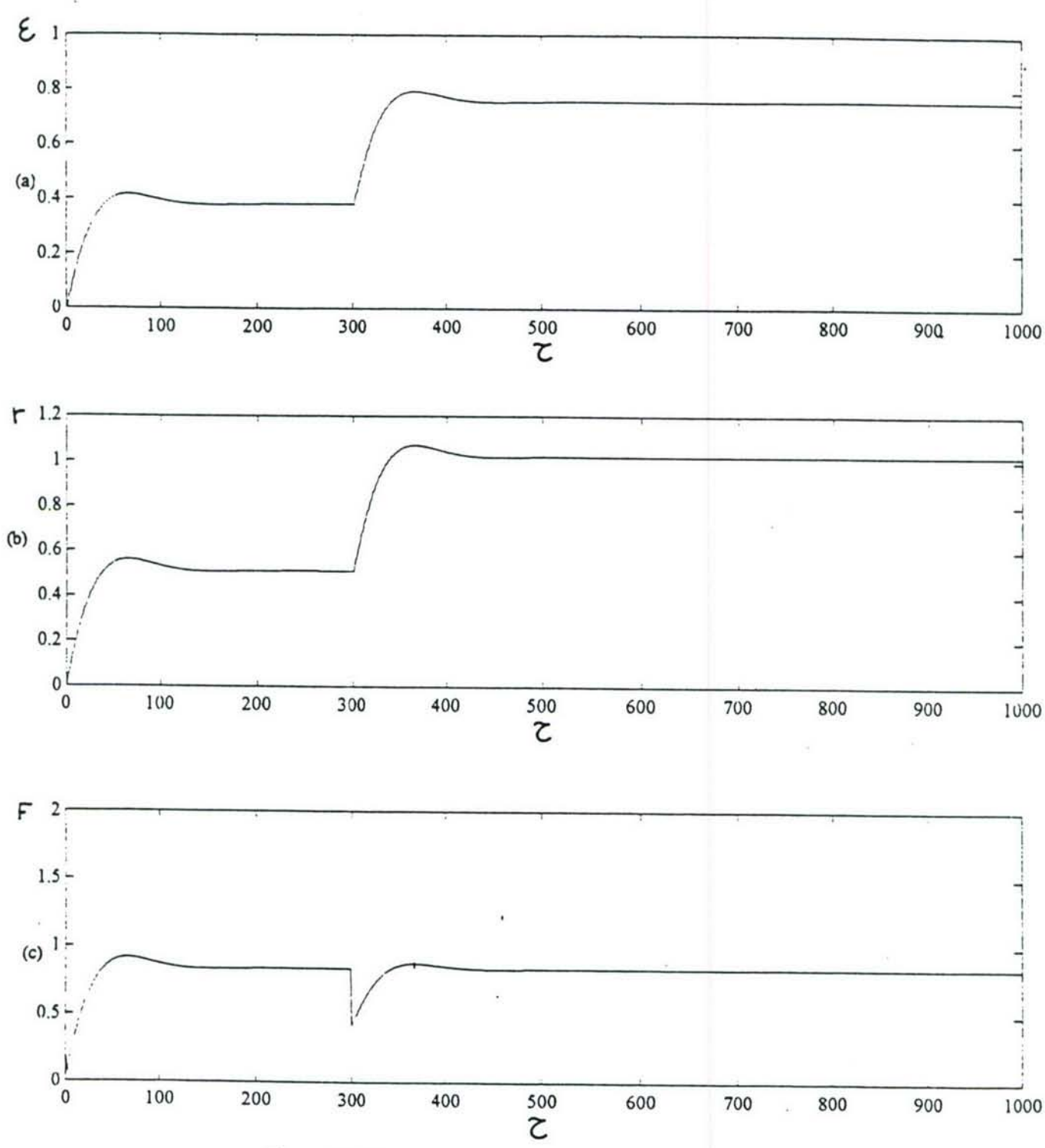
Figure 22 Uncontrolled Response to Sudden Imbalance
