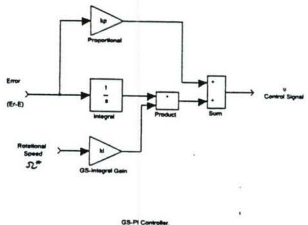
Figure 25 Block diagram of the closed loop system with GS-PI controller.
