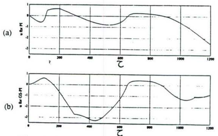
Figure 27 Transient behavior of the control input u for both PI controller case (a), and GS-PI case (b).
