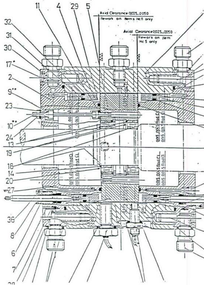
Figure 2 Cut-Out In The Manufactured HSFD
