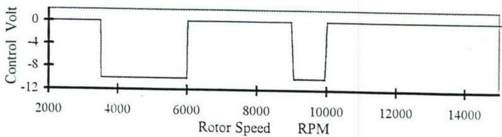
Figure 14 Actuating signal for On/Off controller
