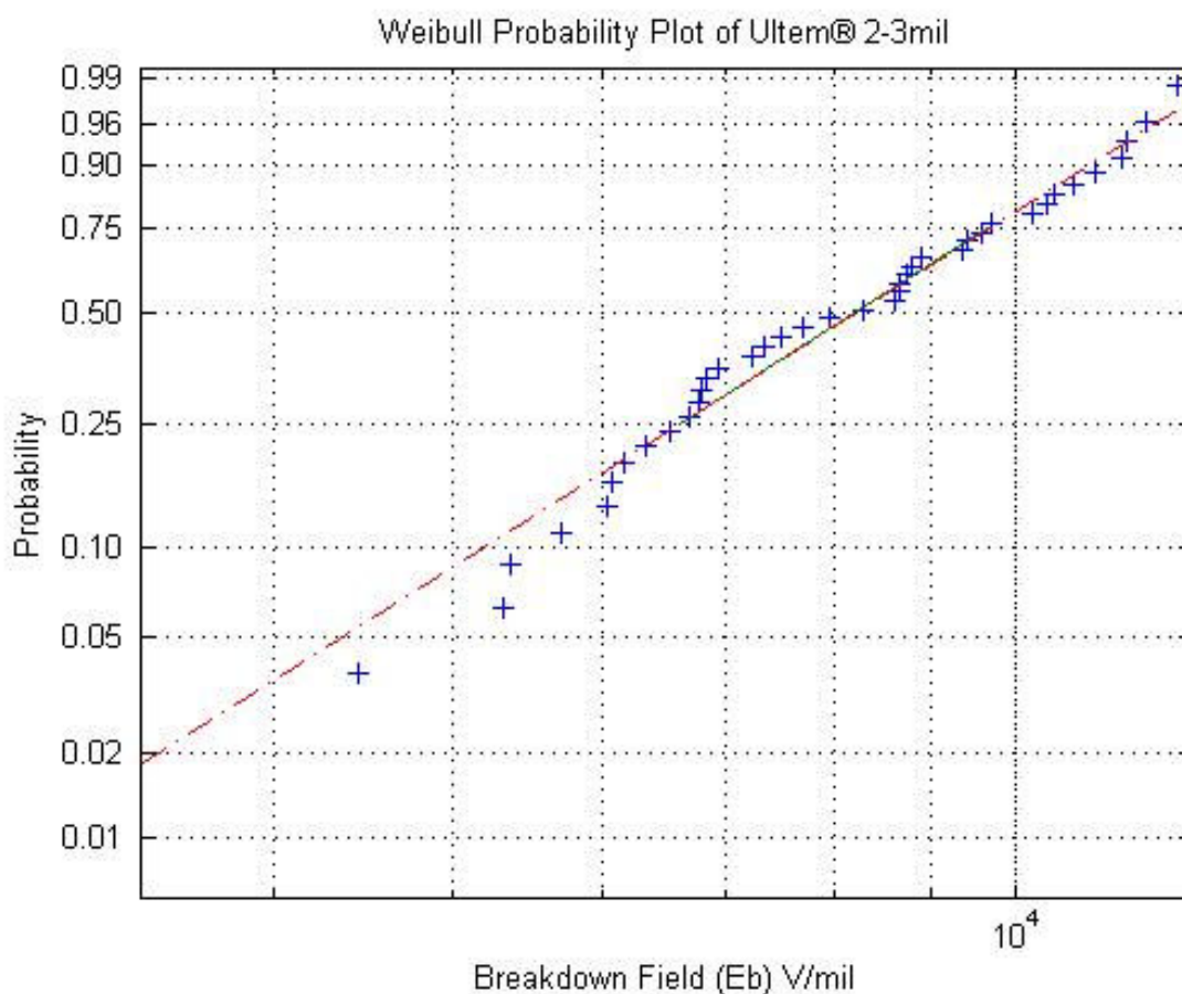
Figure 25: Weibull Cumulative Probability of Failure Plot of Ultem® 2-3 mil as a Function of Electric Field
