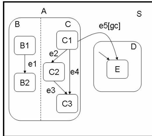
Figure 36 - Multimodel Structure
