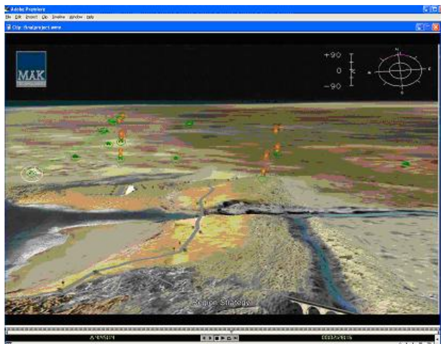
Figure 29 - Region Strategy
