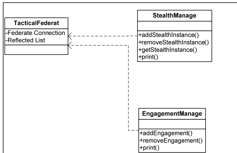
Figure 25 - Stealth Manager
