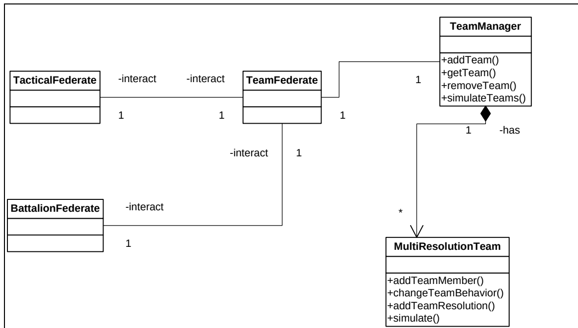
Figure 23 – Team Federate
