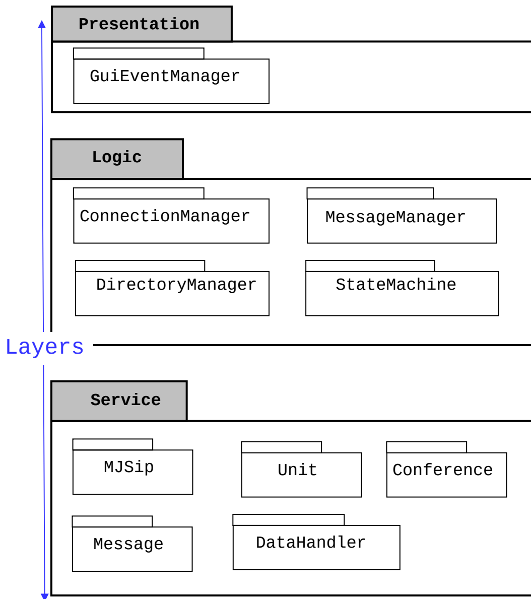
Figure 17. VoIPNET Architecture
