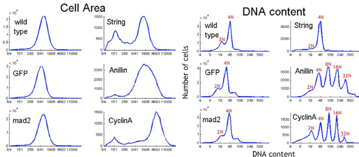
Figure 2: Images from slides with the indicated gene knocked down by RNA interference were analyzed using CellProfiler software to create histograms of cell area (left) and DNA content (right). The results are consistent with existing literature, validating the software.
