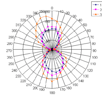
Figure 6c. Radar plot of signal vs. analyzer angle, used to determine rho.
