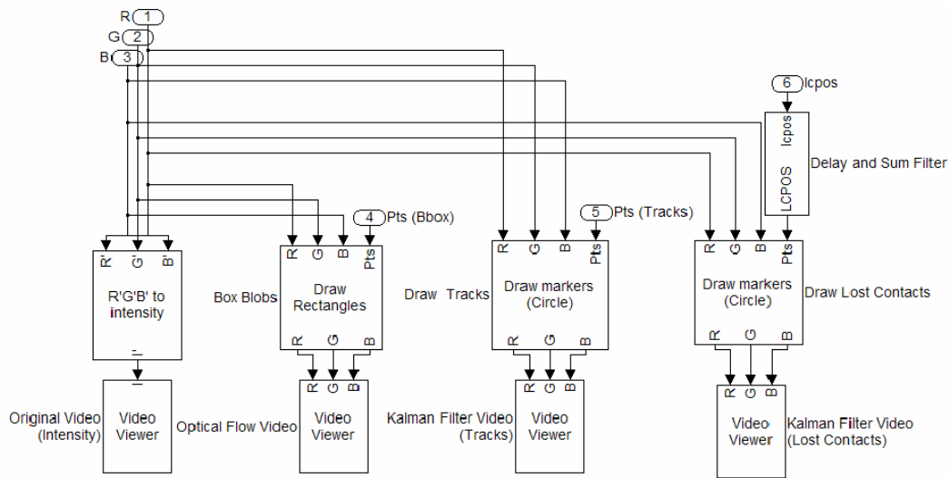
Figure 22. Simulink Block Diagram of Post-Processing Subsystem
