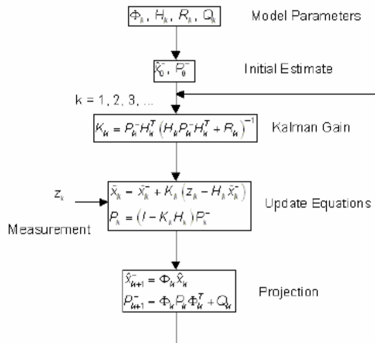
Figure 3. Kalman Filter Recursion [From Ref.7]
