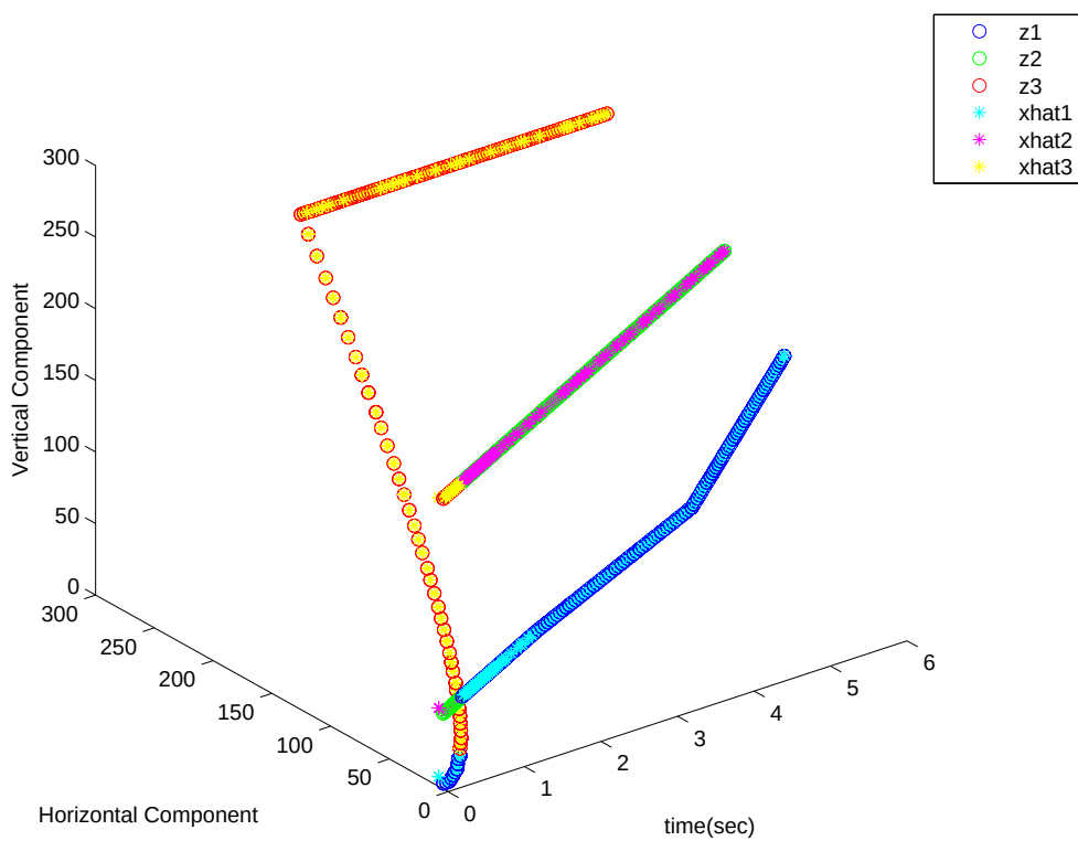
Figure 31. Position Tracks for Multiple Contacts under Various Conditions
