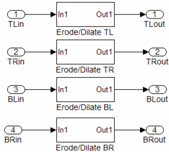
Figure 16. Simulink Block Diagram of Erosion and Dilation Subsystem
