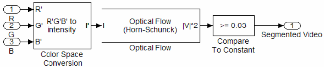
Figure 5. Simulink Block Diagram of Segmentation Subsystem
