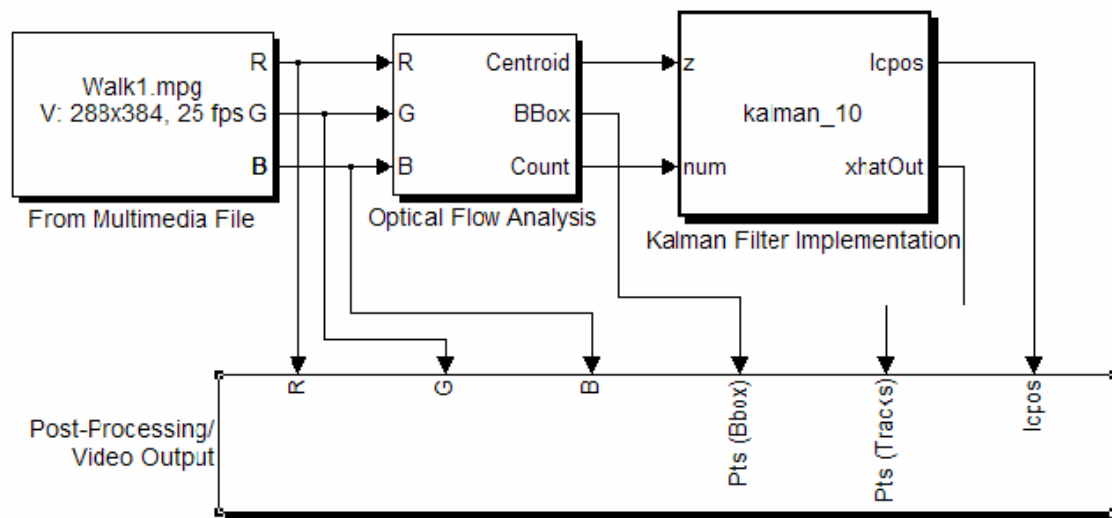
Figure 1. Simulink Block Diagram of Surveillance Video Processor
