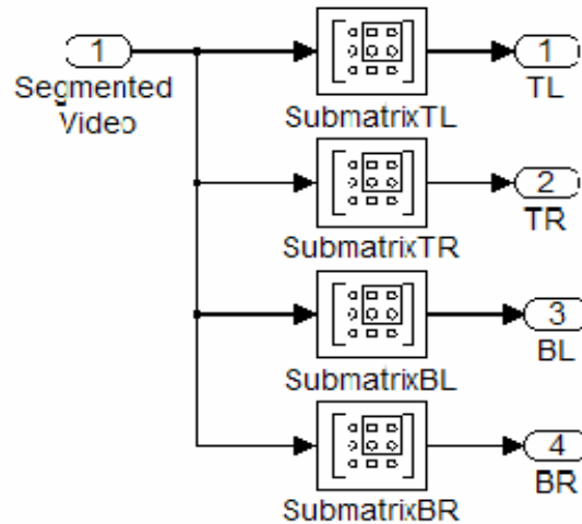
Figure 14. Simulink Block Diagram of Quadrant Operation Subsystem
