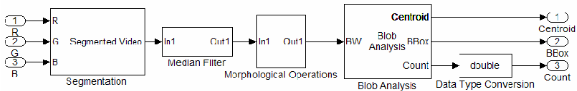
Figure 4. Simulink Block Diagram of Optical Flow Subsystem
