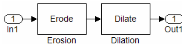
Figure 17. Simulink Block Diagram of a Erosion and Dilation Subsystem for a Particular Quadrant
