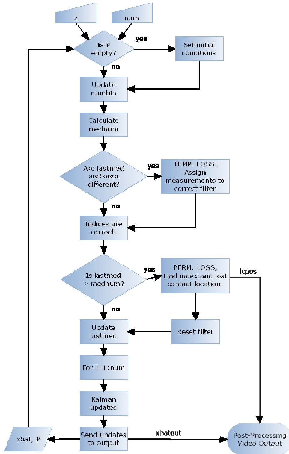
Figure 21. Flow Diagram for Embedded MATLAB Function Kalman Filter Implementation
