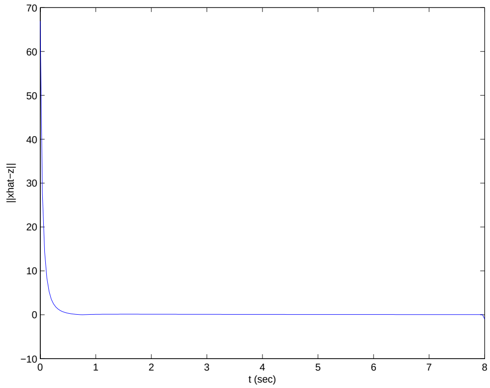
Figure 28. Vector Norm Plot for One Contact (Constant Speed and Varying Direction)
