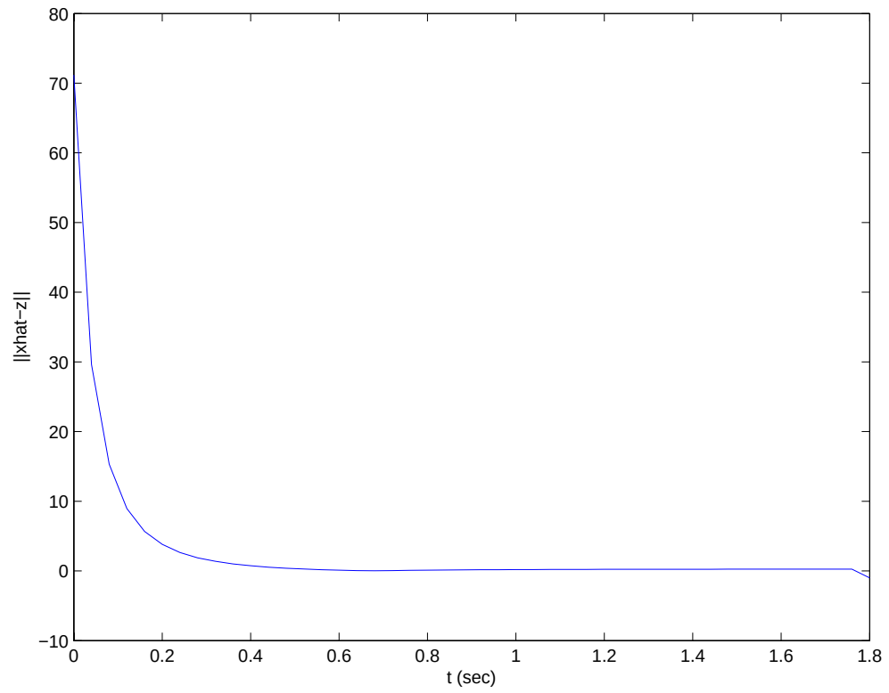
Figure 26. Vector Norm Plot for One Contact (Varying Speed and Constant Direction)
