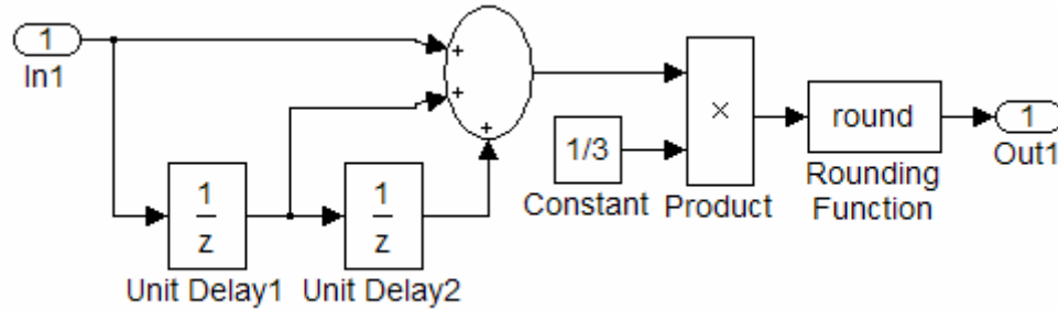
Figure 10. Simulink Block Diagram of Median Filter Implementation
