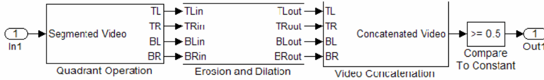
Figure 13. Simulink Block Diagram of Morphological Operations Subsystem
