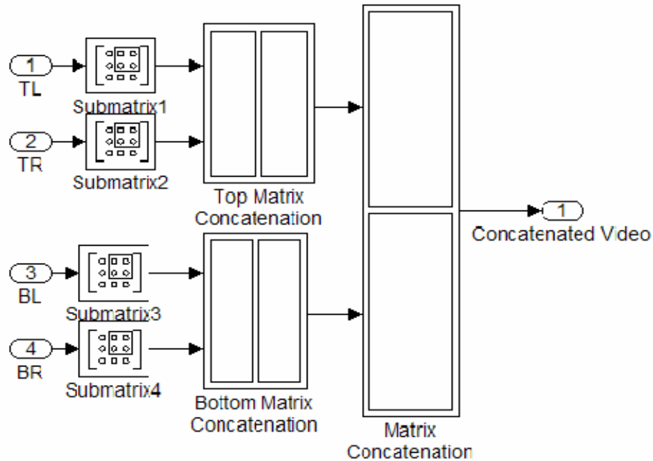
Figure 18. Simulink Block Diagram of Video Concatenation Subsystem
