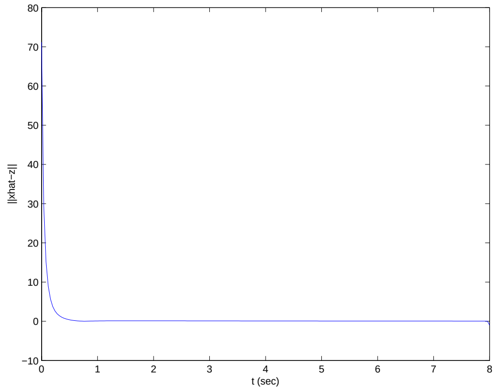
Figure 24. Vector Norm Plot for One Contact (Constant Speed and Direction)
