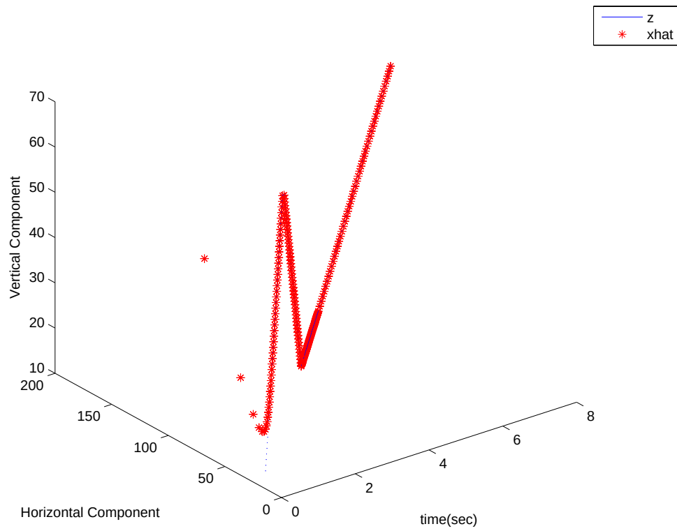
Figure 29. Position Track for One Contact (Constant Speed and Varying Direction)
