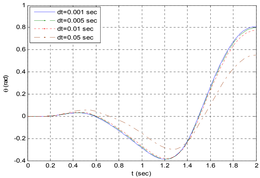
Figure 105. Convergence evaluation for forced oscillation – no jumps
