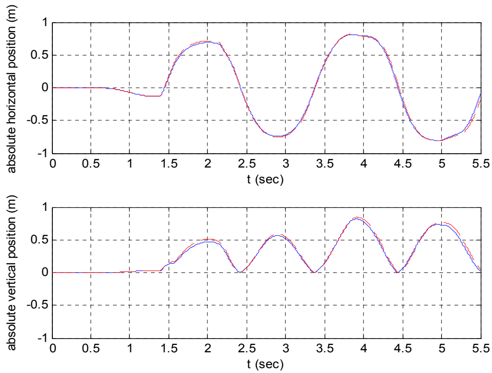
Figure 103. Mass absolute position
