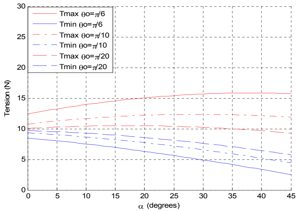
Figure 35. Maximum and minimum tensions
