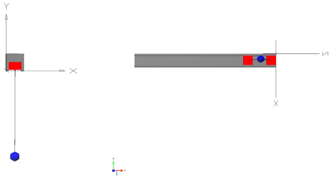
Figure 41. Side and bottom view of 2-pendulum VN 4-D model
