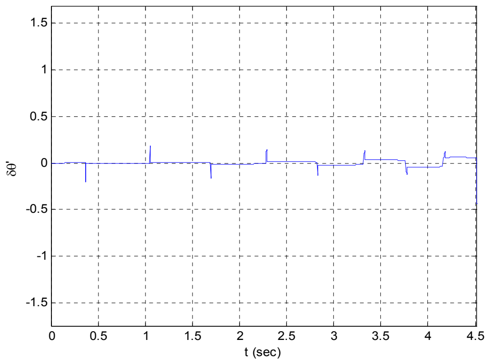
Figure 60. Prediction discrepancy
