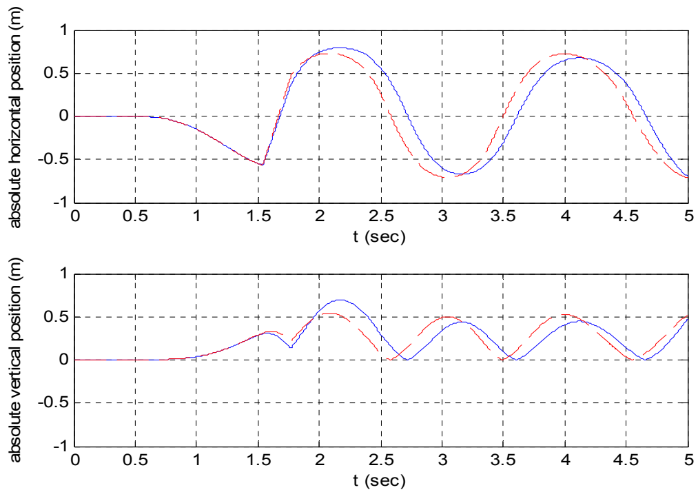
Figure 98. Mass absolute position
