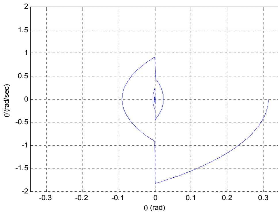
Figure 70. Phase diagram
