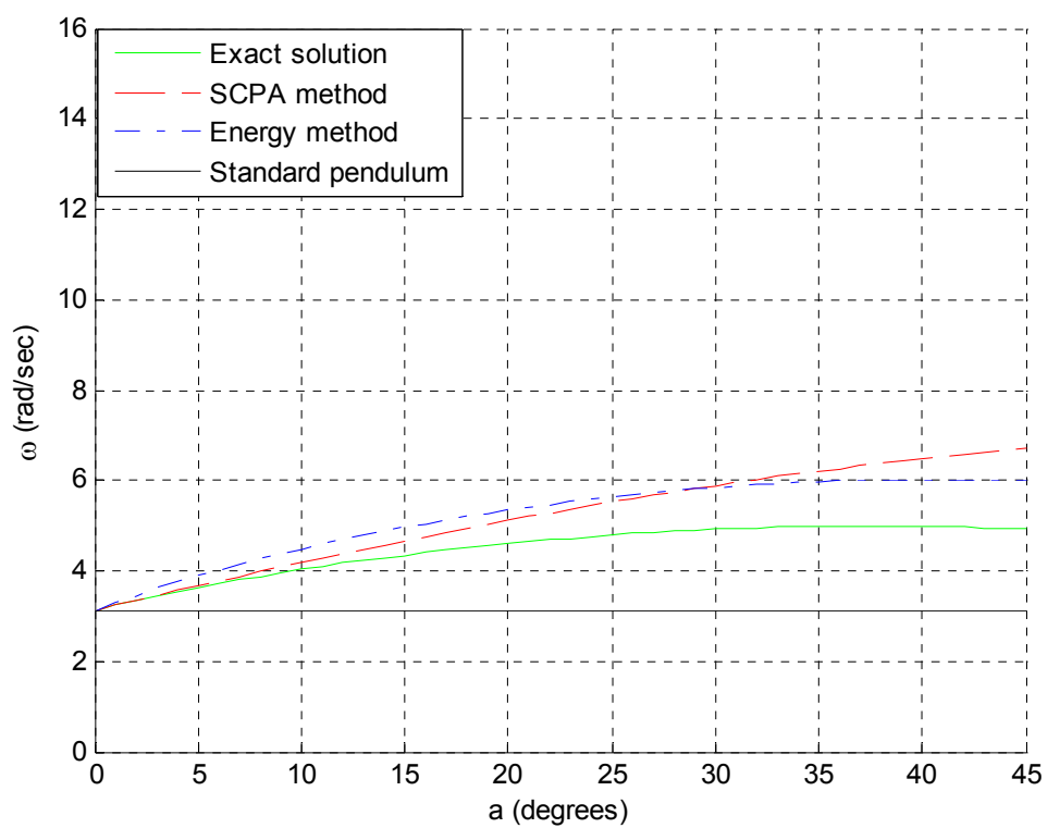
Figure 29. \theta_0 = \pi/10
