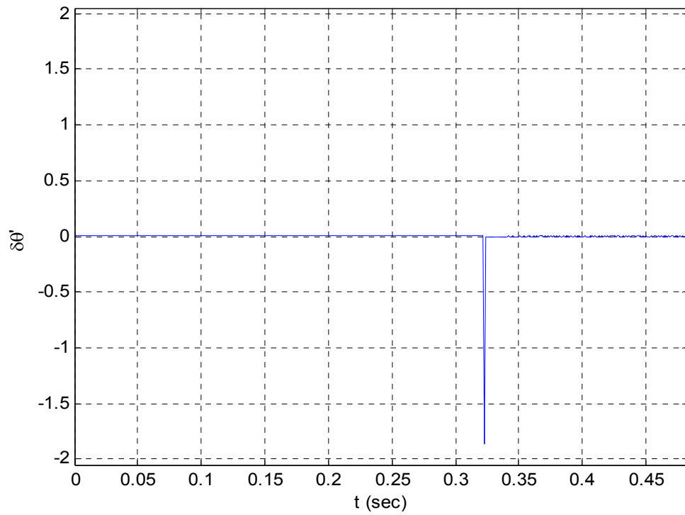
Figure 79. Prediction discrepancy
