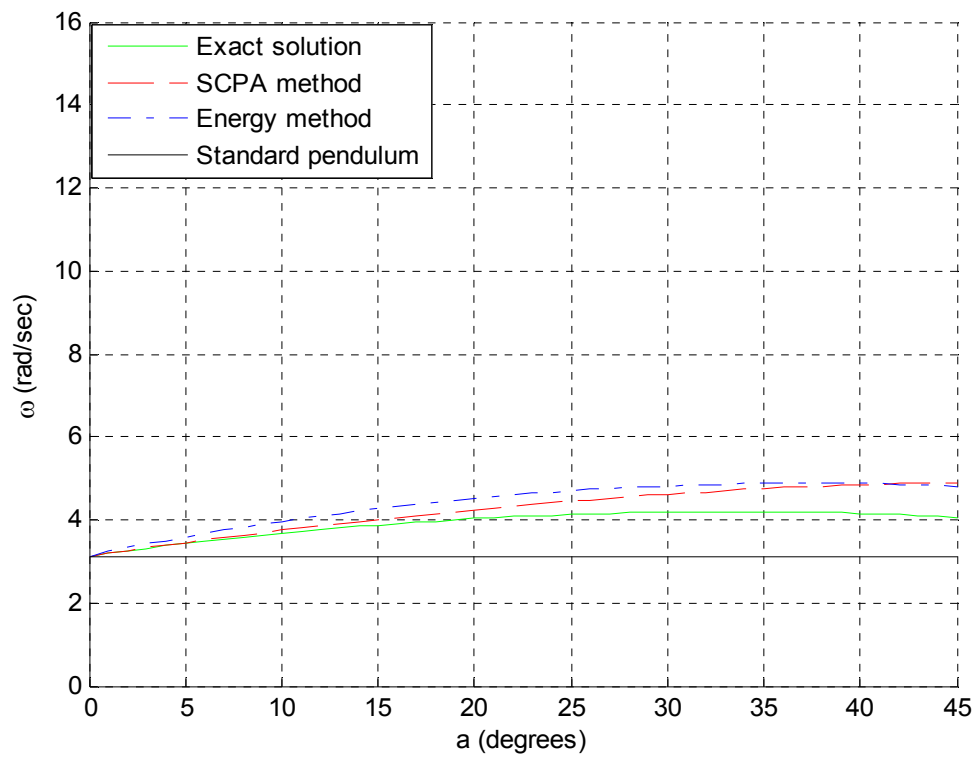
Figure 28. \theta_0=\pi/6
