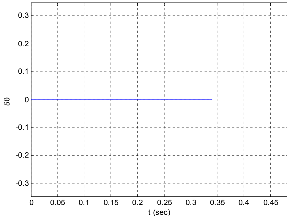
Figure 76. Prediction discrepancy
