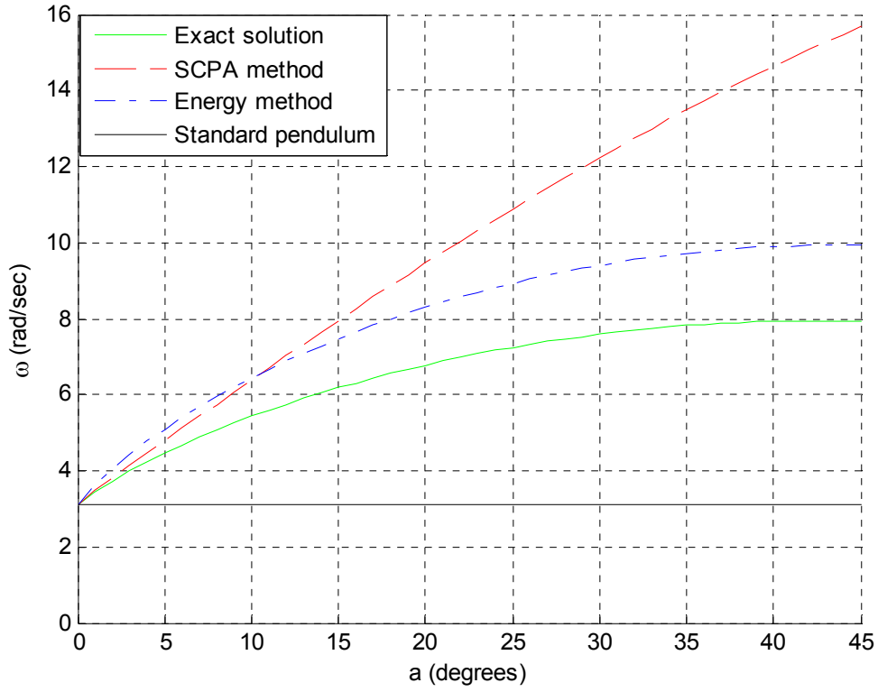
Figure 31. \theta_0 = \pi/30
