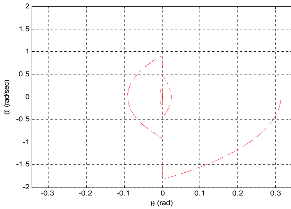
Figure 69. Phase diagram
