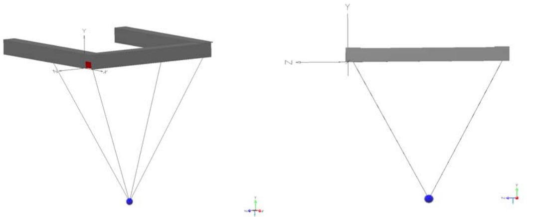
Figure 107. 4-pendulum perspective and front view
