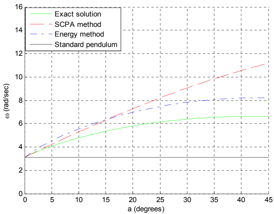
Figure 30. \theta_0 = \pi/20
