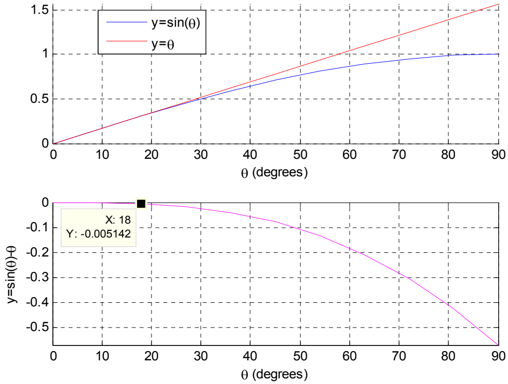
Figure 3. Linear-nonlinear discrepancy
