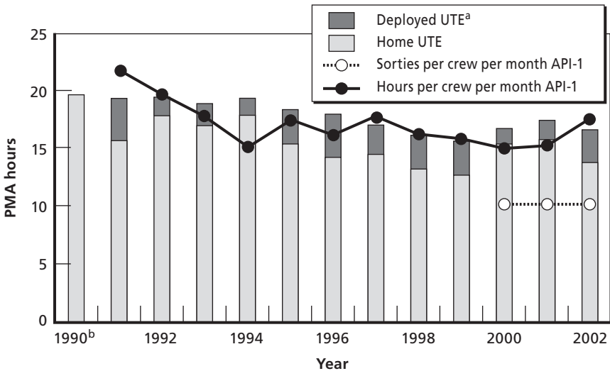
Figure 2.2 Air Combat Command F-15A/C UTE, Hours, Sorties Comparison
