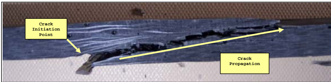
Figure 25. Crack Initiation and Propagation (Base)
