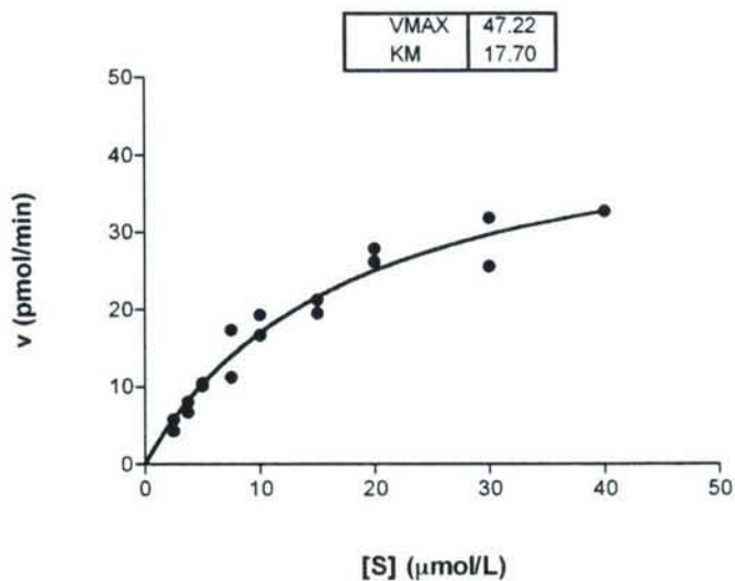
Lineweaver-Burk Plot
