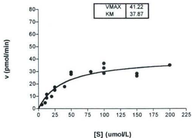
Lineweaver-Burk Plot
