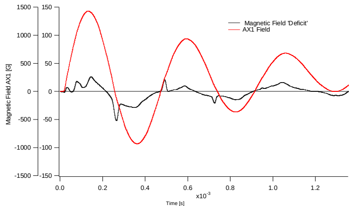
Figure 12. Magnetic field deficit for a 500V 14 mTorr discharge
