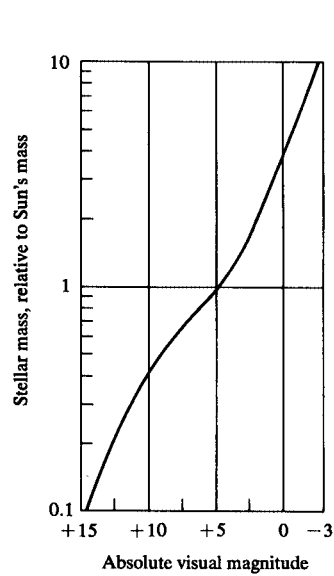
Figure 32. Absolute visual magnitude of main-sequence stars as a function of stellar mass.
