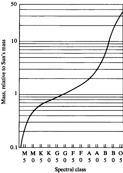
Figure 33. Mass as a function of spectral class (main-sequence stars).
