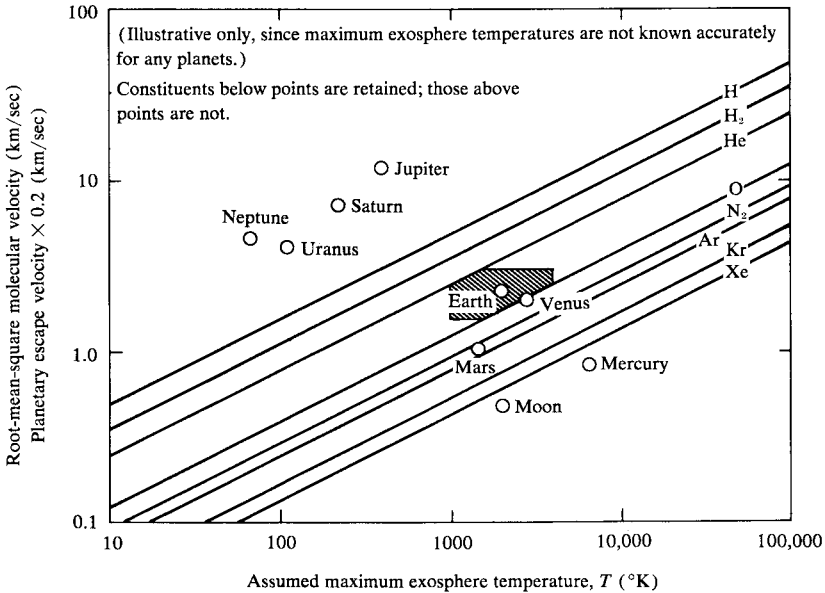
Figure 12. Planetary atmospheres.
