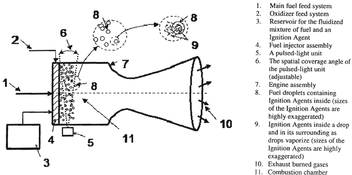
Figure 3 Schematic diagram showing an application of the SWCNTs as ignition agents for the ignition process in a liquid rocket engine combustion chamber (drawing not to scale).
