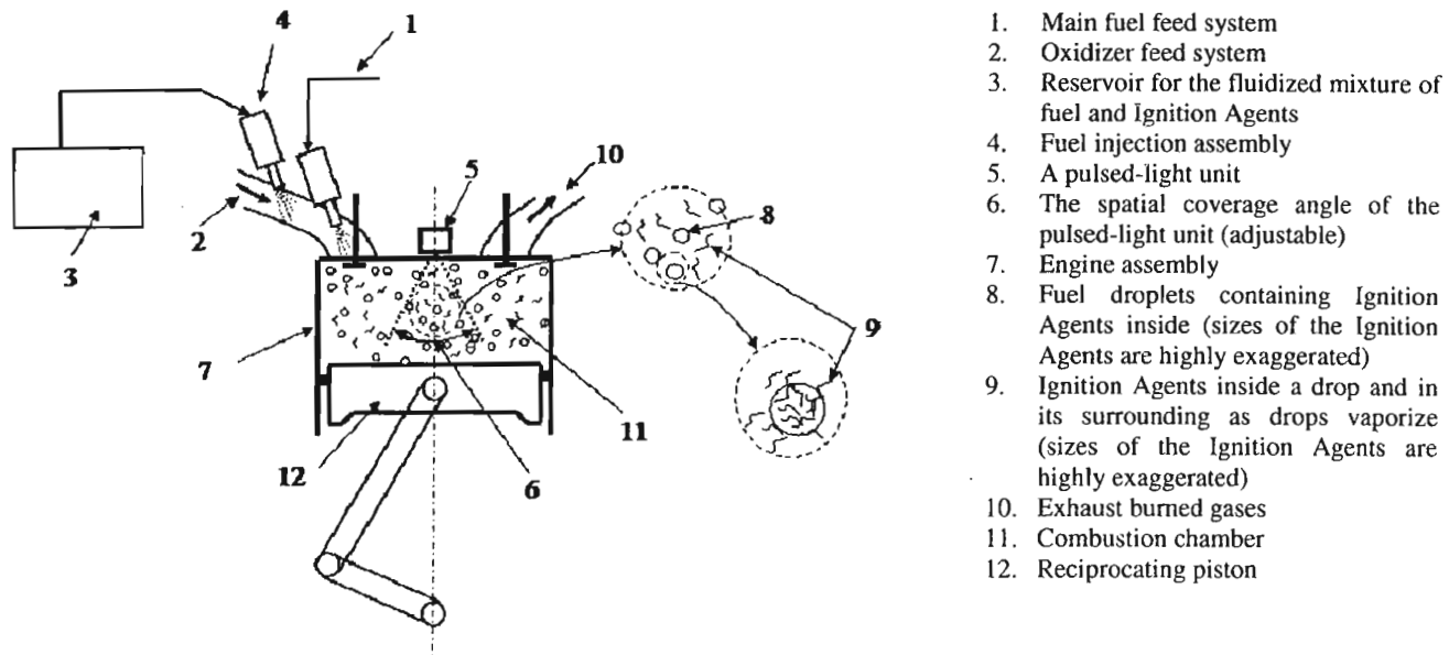
Figure 4 Schematic diagram showing an application of the SWCNTs as ignition agents for the ignition process in a reciprocating combustion engine (drawing not to scale).
