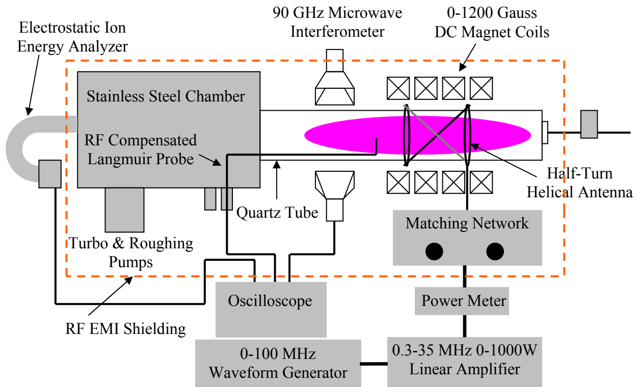
Figure 5. Schematic of AFRL Experimental Helicon research station.
