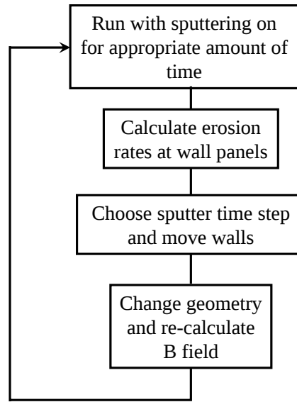
Figure 10. Erosion model flow chart.
