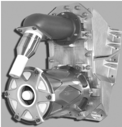
Figure 11. BHT-200 thruster.
