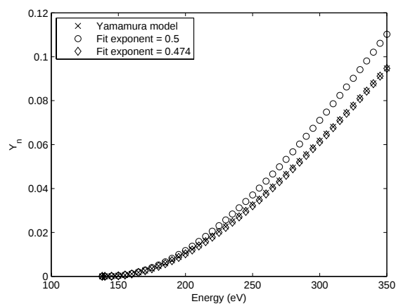
Figure 4. Comparison of Yamamura model to Equations 4 and 5, boron.
