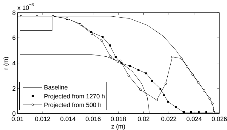
Figure 19. BHT-200 projected end of life profiles (1,330 h).
