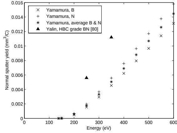
Figure 3. Comparison of \text{Xe}^+ \rightarrow \text{BN} analytical and experimental normal sputter yields.
