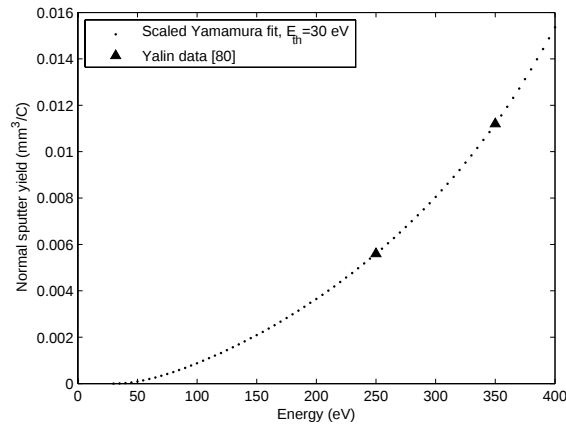
Figure 6. Yield fit for E_{th}=30 eV.
