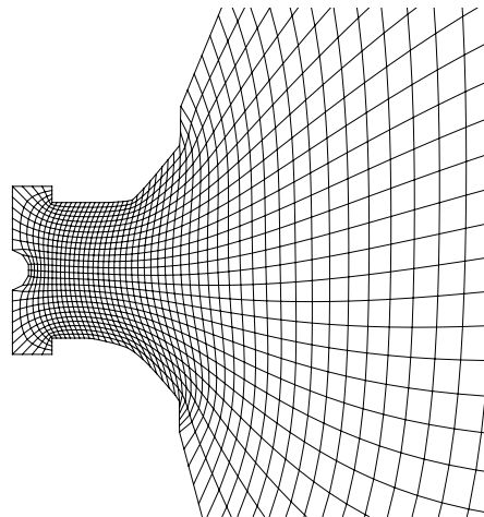
Figure 17. BHT-600: Detail of initial mesh after 80 hours of operation.
