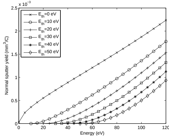
Figure 7. Near-threshold region yield fits.
