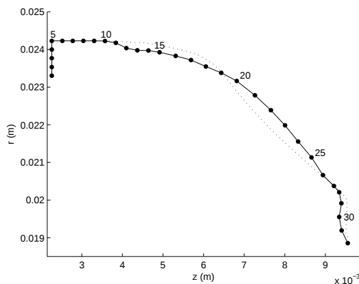
(c) Inner insulator, 494 hours.
