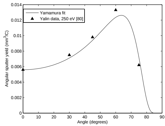
Figure 8. Yamamura-based angular sputter yield model, 250 eV.
