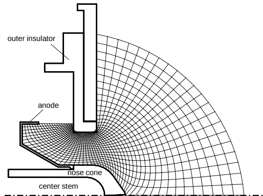
Figure 12. Initial BHT-200 geometry.
