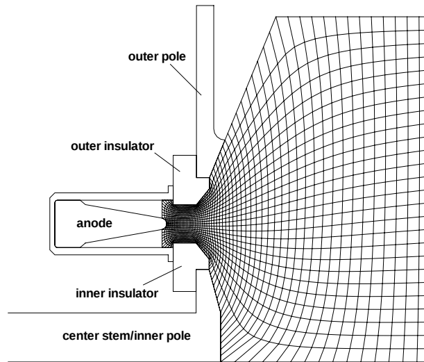
Figure 16. BHT-600 geometry.
