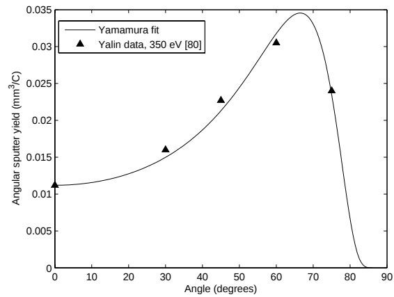
Figure 9. Yamamura-based angular sputter yield model, 350 eV.
