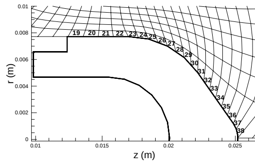
Figure 13. Detail of BHT-200 nose cone panels.
