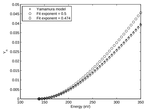
Figure 5. Comparison of Yamamura model to Equations 4 and 5, nitrogen.
