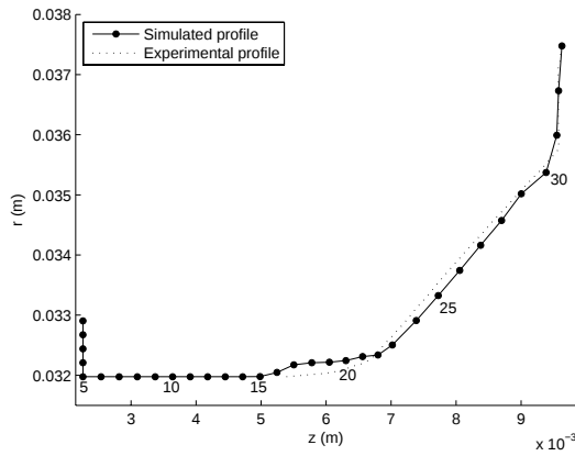
(a) Outer insulator, 494 hours.
