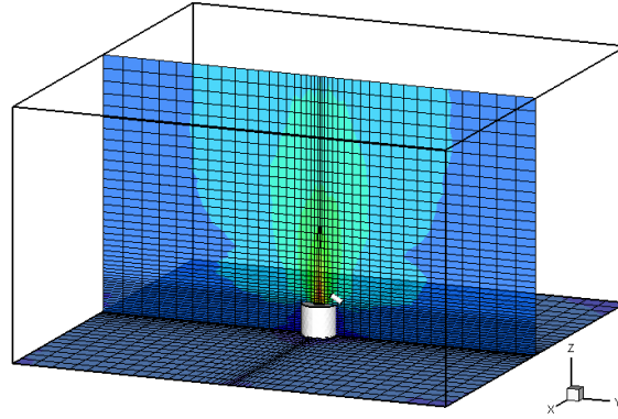
Figure 13. Simulation domain and the thruster geometry. Simulation was performed using a stretched mesh.
