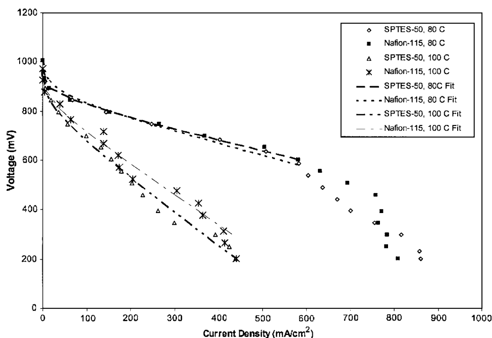
Figure 6. Polarization plots (data and fit) of Nafion and SPTEs-50 using H_2 and air at different temperatures.
