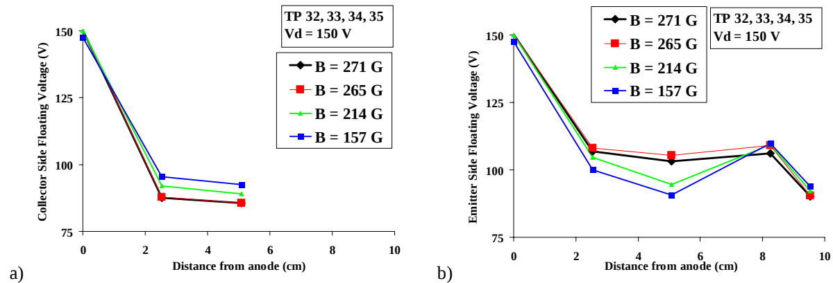
Figure 13. Floating voltages for V_d = 150 (V) and various magnetic field strengths for the a) collector and b) emitter side of the channel.
