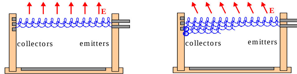
Figure 6. Ideal operation (left) versus non-ideal operation (right).
