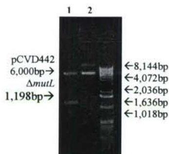
Figure 2. Agarose Gel of pCVD442L Digested with Xma I. Lane 1: pCVD442 (6,000bp) and \Delta mutL (1,198 bp), lane 2: pCVD442, mw, 1 Kb DNA Ladder.
