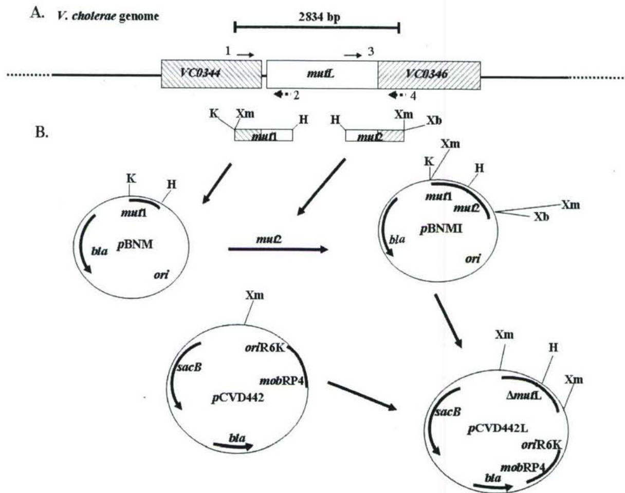
Figure 1. Construction and Cloning of \Delta mutL , an Allele of mutL from V. cholerae Strain N16961 Containing an Internal Deletion. A. Physical map of mutL and flanking genes. Shaded boxes indicate the genes flanking mutL . Solid arrows indicate placement of forward primers. Dotted arrows indicate placement of reverse primers. Numbers correspond to primer sequences located in the table. K: KpnI , H: HindIII , Xm: XmaI , Xb: XbaI . The bar above genome indicates the size of the fragment produced in the intact genome, using primers 1 and 4 from the table. Genes are not drawn to scale. B. Construction of suicide vector pCVD442L, which contains a truncated version of mutL from V. cholerae N16961. Plasmid pBNM was created by amplifying a fragment of the V. cholerae genome containing the 3' end of VC0344 and the 5' end of mutL , digesting the fragment and pBluescript with KpnI and HindIII , ligating, and selecting for ampicillin resistant colonies in E. coli XL1Blue cells. Similarly, pBNMI was created by amplifying a fragment of the V. cholerae genome containing the 3' end of mutL and the 5' end of VC0346, digesting the fragment and pBMN with HindIII and XbaI , ligating, and selecting for ampicillin resistant colonies in XL1Blue. The \Delta mutL fragment was created by cutting pBMNI with XmaI and joining the 1.2-kb fragment with the XmaI -digested plasmid pCVD442, which contains the sacB gene of B. subtilis and the bla gene. The resulting suicide vector was selected by ampicillin resistance in E. coli SM17 \lambda pir cells. Plasmids are not drawn to scale.
