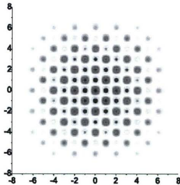
Fig. 20: The fundamental mode in a finite square array of nanowires (size 13x13) with sides along the symmetry axes of the array. This mode has a high Q of 150,000 and a normalized mode volume of only 8. The Q factor reduces by two orders of magnitude when the sides of the square are oriented at 45 degrees to the symmetry axes.
