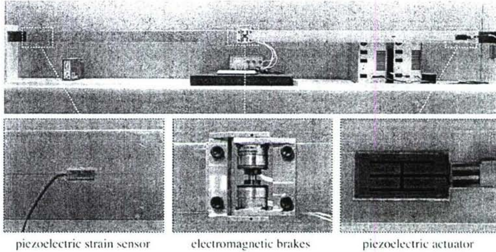
Figure D3. Clamped-clamped beam with mid-span hinge. The hinge is locked and set free by activating and de-activating an electromagnetic brake to change stiffness and demonstrate modal disparity
