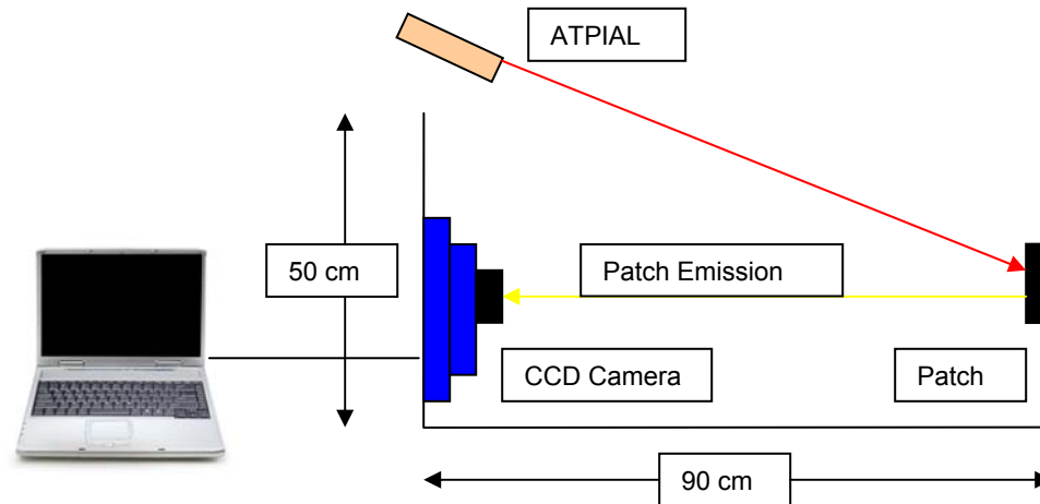
Figure 9. Schematic Drawing of Patch Intensity Testing Apparatus Enclosed in a Wooden Box (not to scale).
