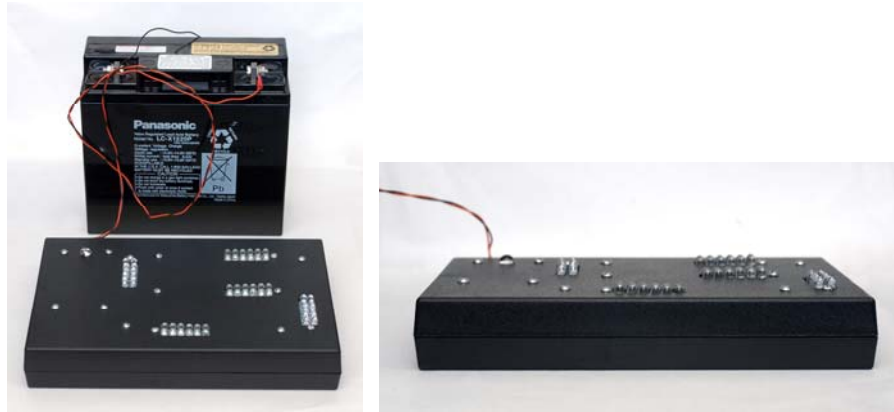
Figure 42. Digital Images of G2 VMIFF with 12 V DC Power Supply.
