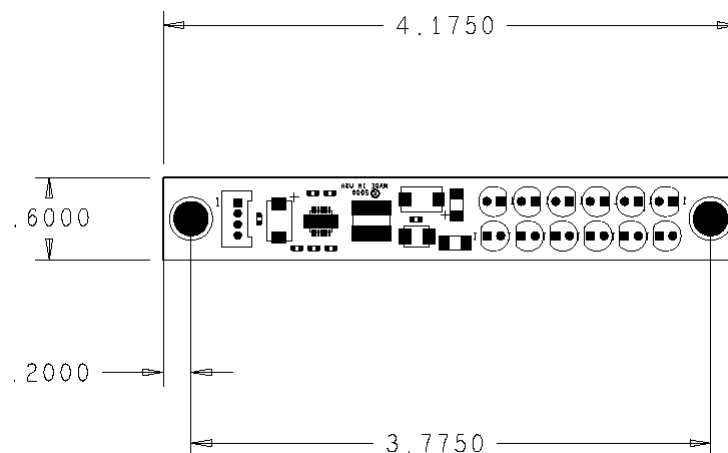
Figure 40. LED Driver and LED Circuit Board Dimensional Drawing (courtesy of Bill Cross).
