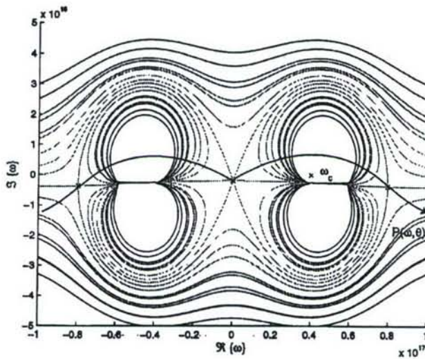
Fig. 3.3 Contours of \Re\{\phi(w, \theta)\} for \theta = \theta_1 in the complex w -plane along with an acceptable deformed path of integration P(w, \theta) . Notice that the original and deformed contours lie on the same side of the pole.
