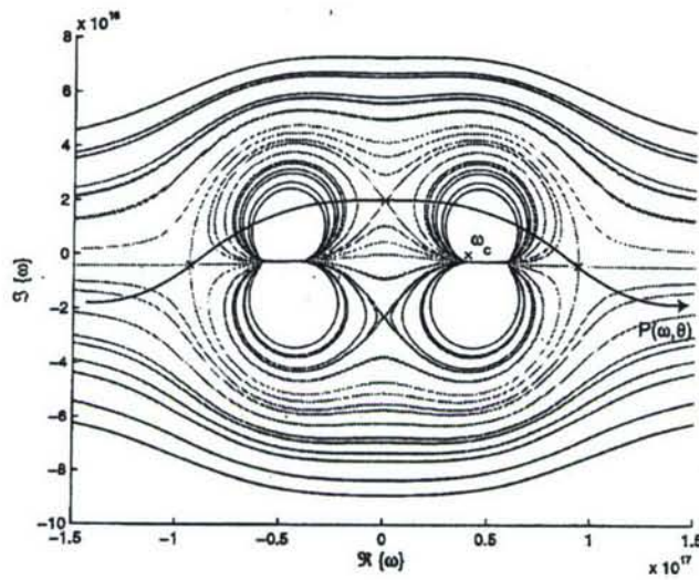
Fig. 3.2 Contours of \Re\{\phi(w, \theta)\} for \theta = 1.25 in the complex w -plane along with an acceptable deformed path of integration P(w, \theta) . Notice that the original and deformed contours lie on the same side of the pole.
