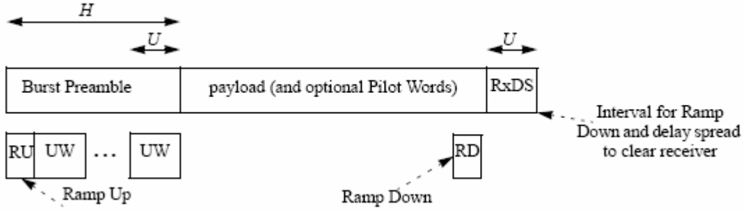
Figure 4 Fundamental Burst Framing Elements (Ref. [11]).
