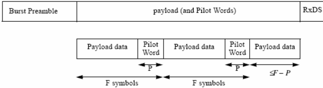
Figure 5 Pilot Word Patterning within a Burst (Ref. [1].)
