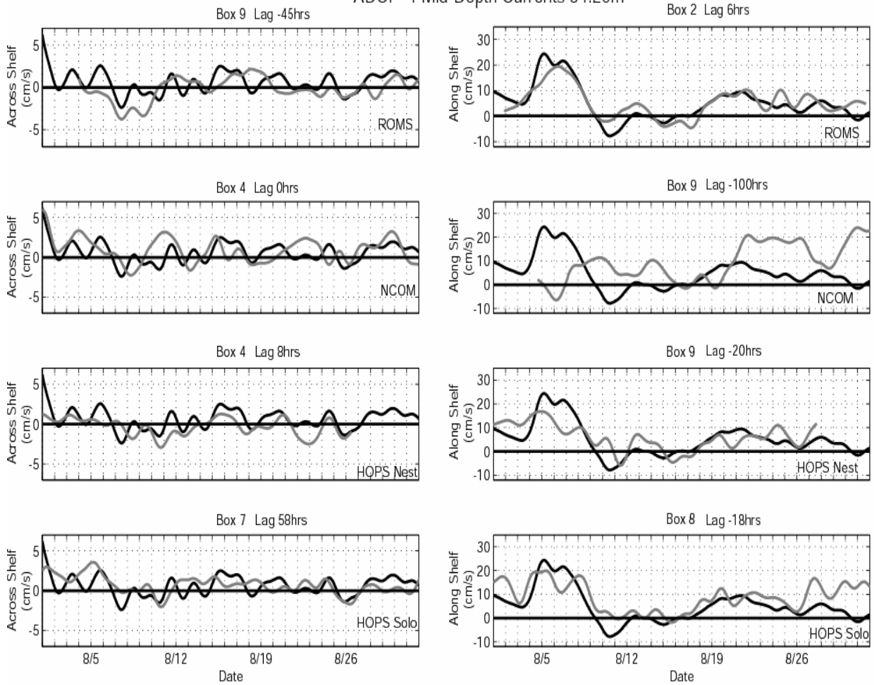
Figure 45. Optimal space/time lagged data producing the highest correlations and minimal rms error between the model output and the data at ADCP 1. For example, the alongshelf ROMS data was best at grid point 2, lagged back by 6 hours.
