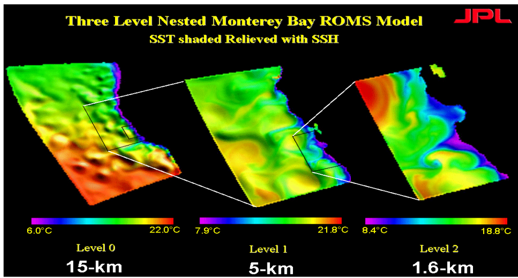
Figure 3. Top: HOPS two way nested modeling scheme (From Pierre Lermusiaux, MIT) Middle: Hierarchy of Navy Coastal Ocean Models (NCOM) in the Pacific (from http://www7320.nrlssc.navy.mil , last accessed May 2007) Bottom: Digital representation of ROMS model nesting depicting a three level one-way nested scheme (From http://ocean.jpl.nasa.gov/MB06/ , last accessed April 2007).
