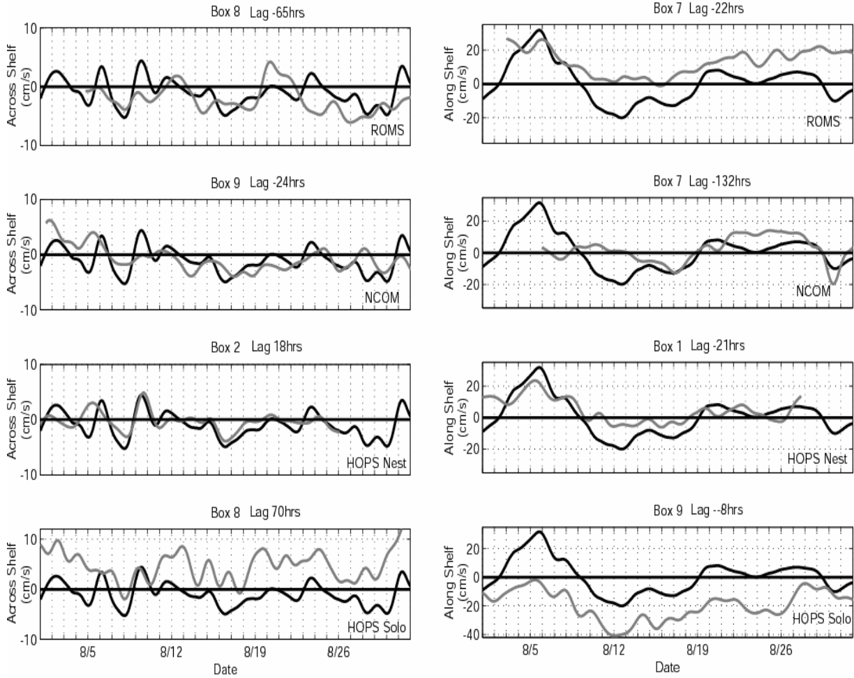
Figure 48. Optimal space/time lagged data producing the highest correlations and minimal rms error between the model output and the data at ADCP 2. For example, the alongshelf ROMS data was best at grid point 7, lagged ahead by 22 hours.
