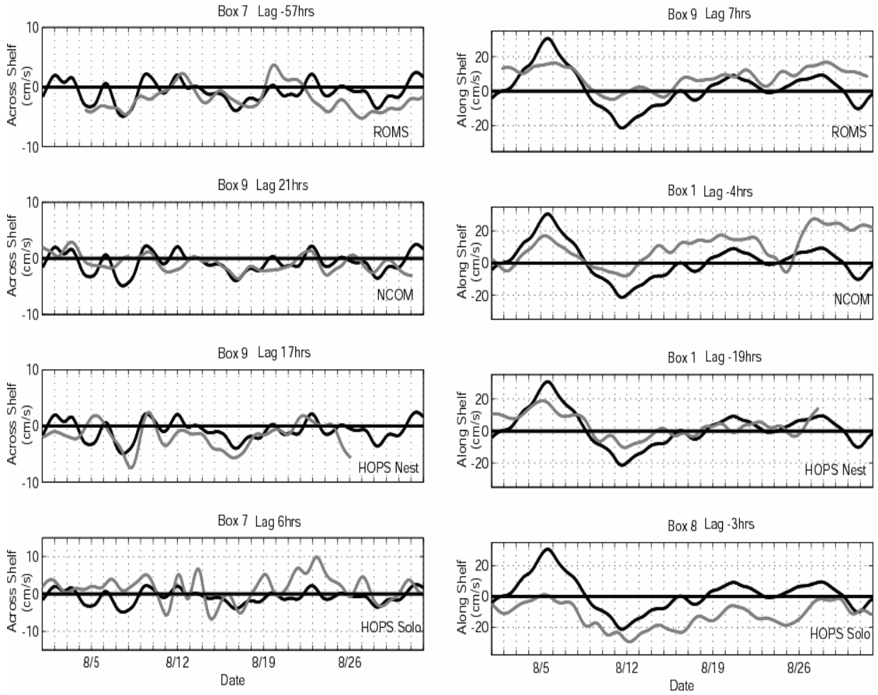
Figure 49. Optimal space/time lagged data producing the highest correlations and minimal rms error between the model output and the data at ADCP 2. For example, the alongshelf ROMS data was best at grid point 9, lagged back by 7 hours.
