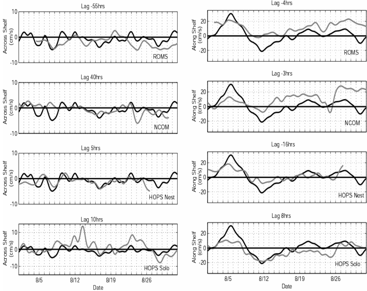
Figure 43. As in Figure 37, but with the series aligned better according to the cross-correlation results. The model output has been shifted forward/back according to the lag/lead estimated from the peak in the cross-correlation function.
