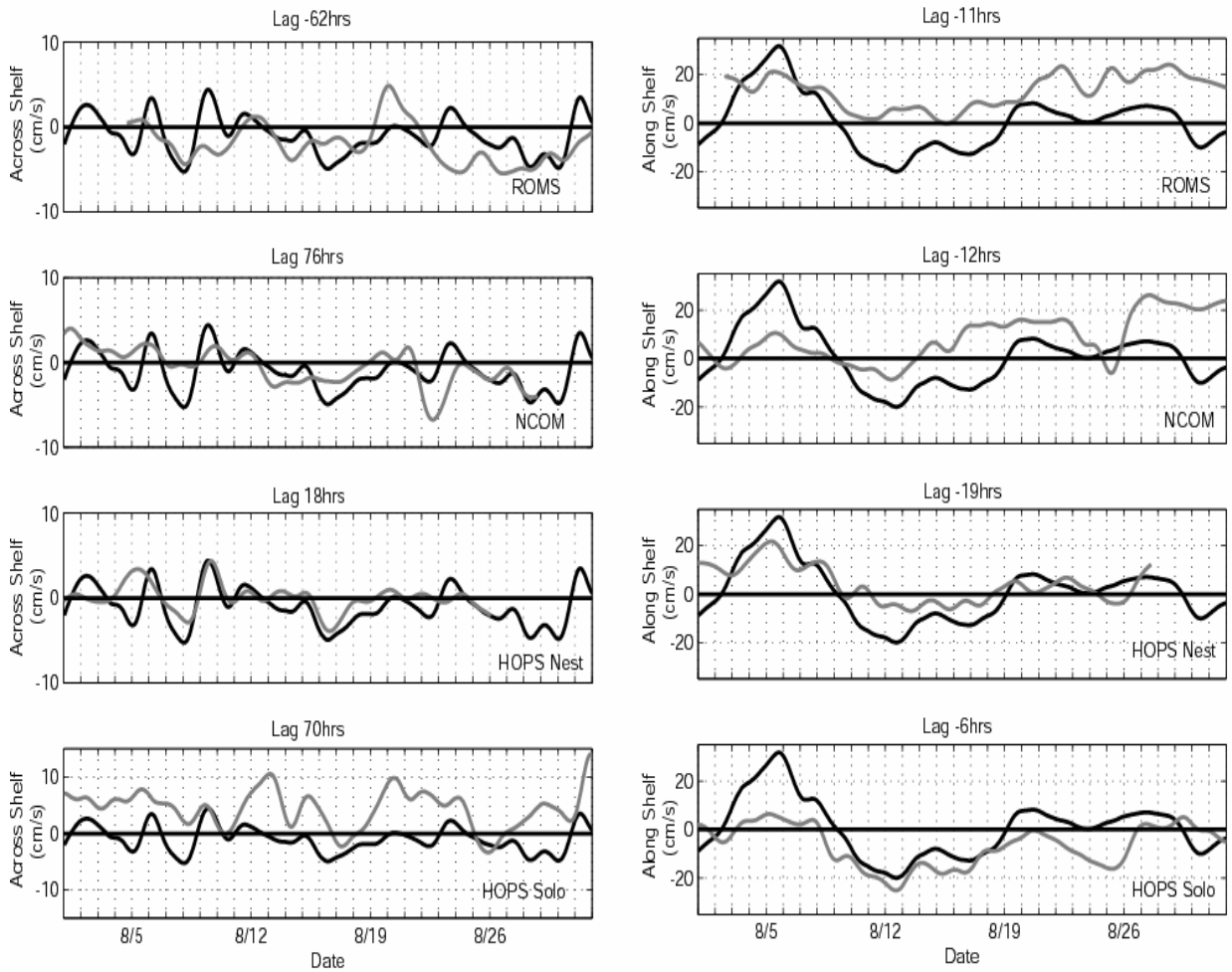
Figure 42. As in Figure 36, but with the series aligned better according to the cross-correlation results. The model output has been shifted forward/back according to the lag/lead estimated from the peak in the cross-correlation function.
