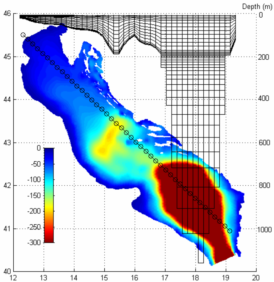
Figure 6. This representation of hybrid vertical levels shows the sigma coordinates at the surface layer and the z coordinates in the deep water and away from abrupt topography. (From Dr. Julie Pullen, Marine Meteorology Division, NRL).
