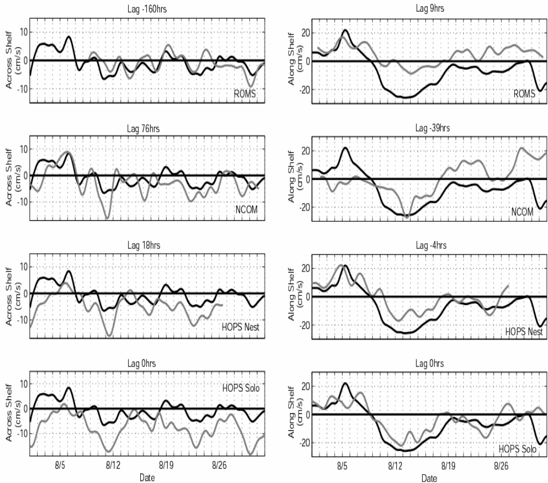
Figure 41. As in Figure 35, but with the series aligned better according to the cross-correlation results. The model output has been shifted forward/back according to the lag/lead estimated from the peak in the cross-correlation function.
