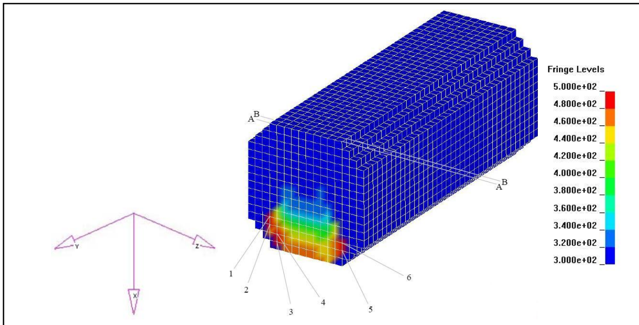
Figure 11. The initial temperature field in the M30A1 grain and the six-nodes and two-faces (A and B) for which temperature histories are recorded in figure 12 (4).
