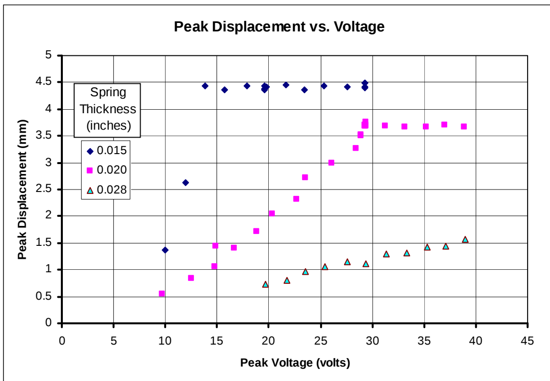
Figure 6. Peak displacement vs. voltage.
