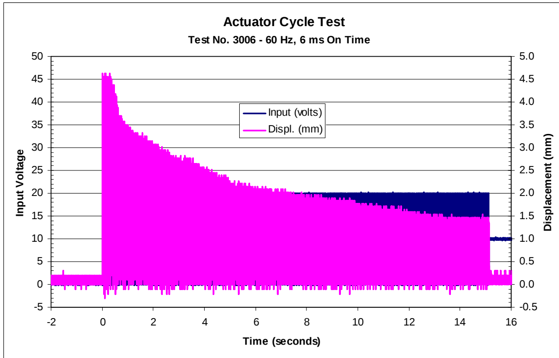
Figure 12. Stress test of multiple 20 V, 6 ms pulses, 0.015 in. spring.
