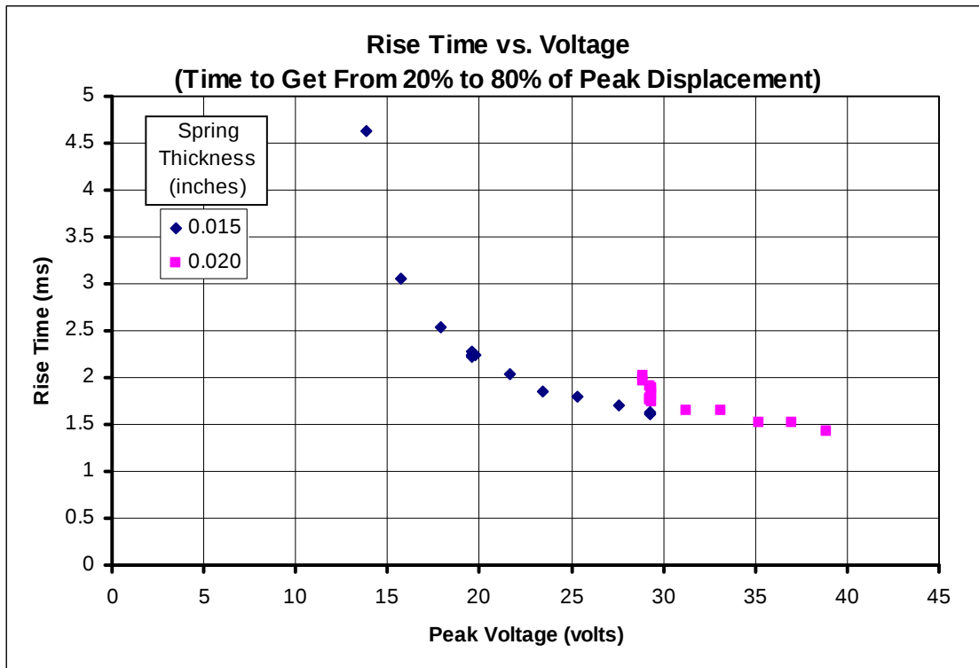
Figure 7. Rise time vs. voltage.
