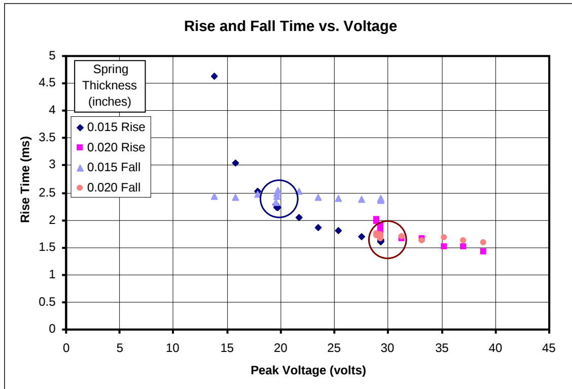
Figure 9. Combined rise and fall time measurements.
