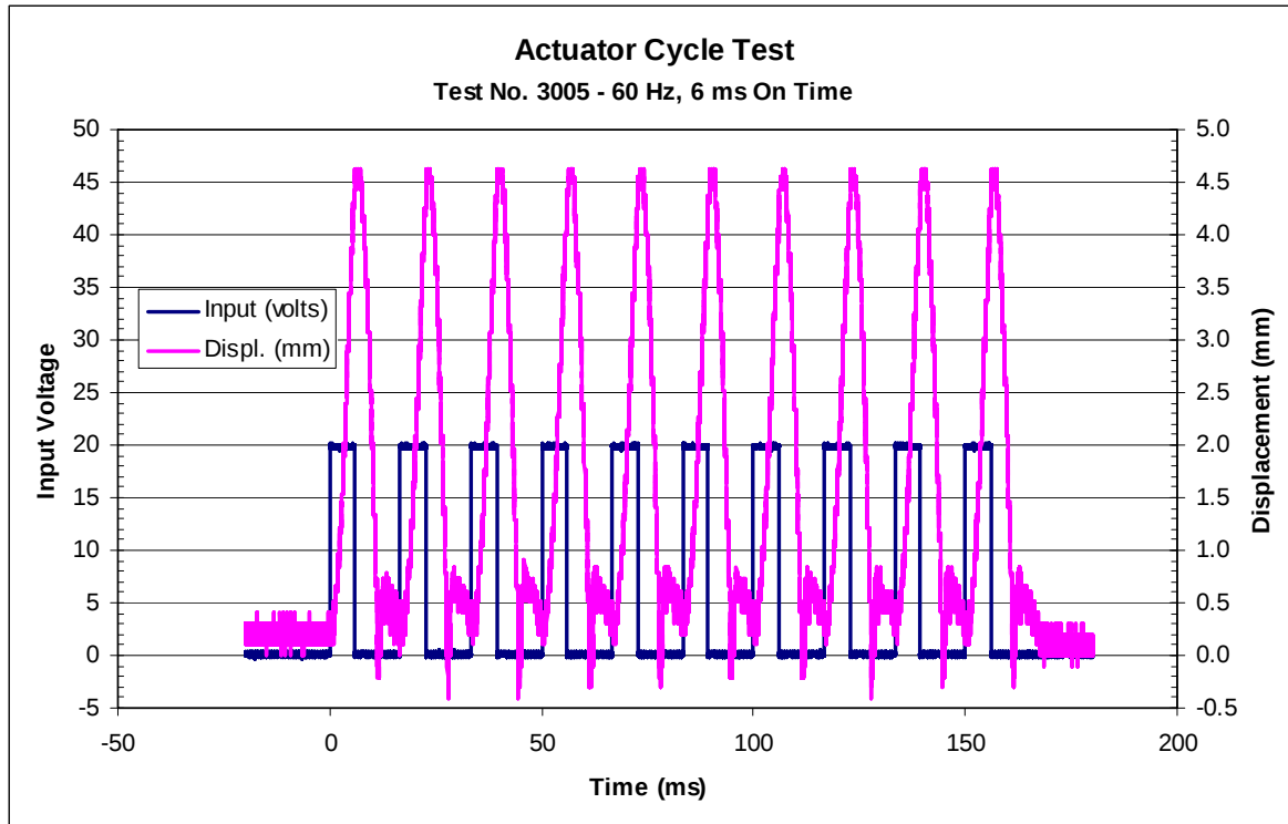
Figure 11. Series of ten 20 V, 6 ms pulses, 0.015 in. spring.
