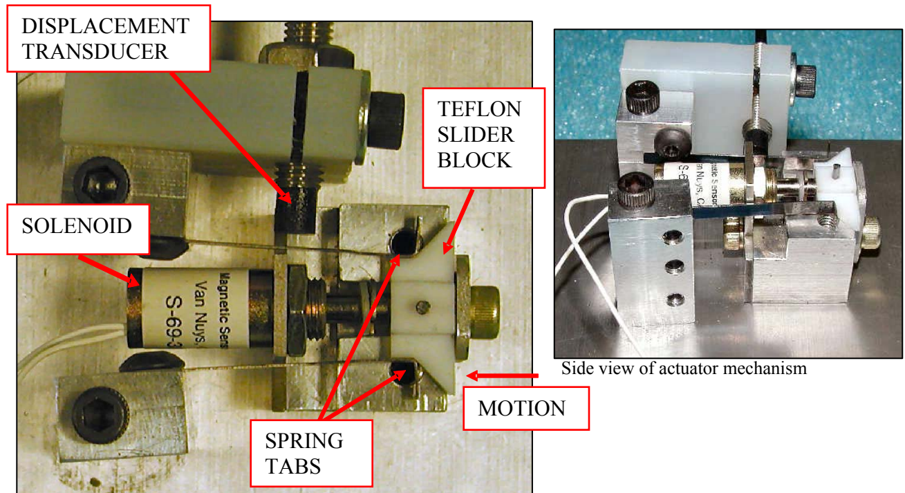
Figure 4. Actuator mechanism test fixture.
