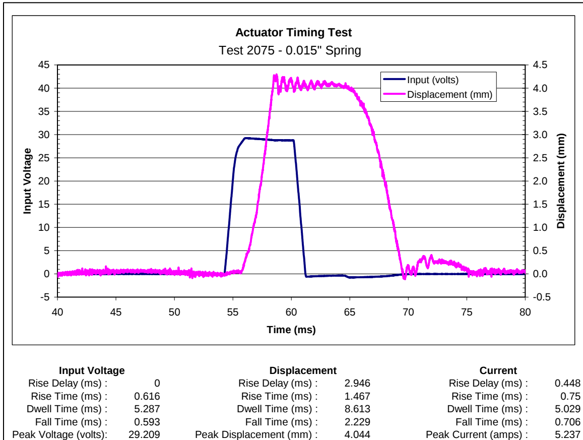
Figure 5. Sample result from a single pulse actuation test.
