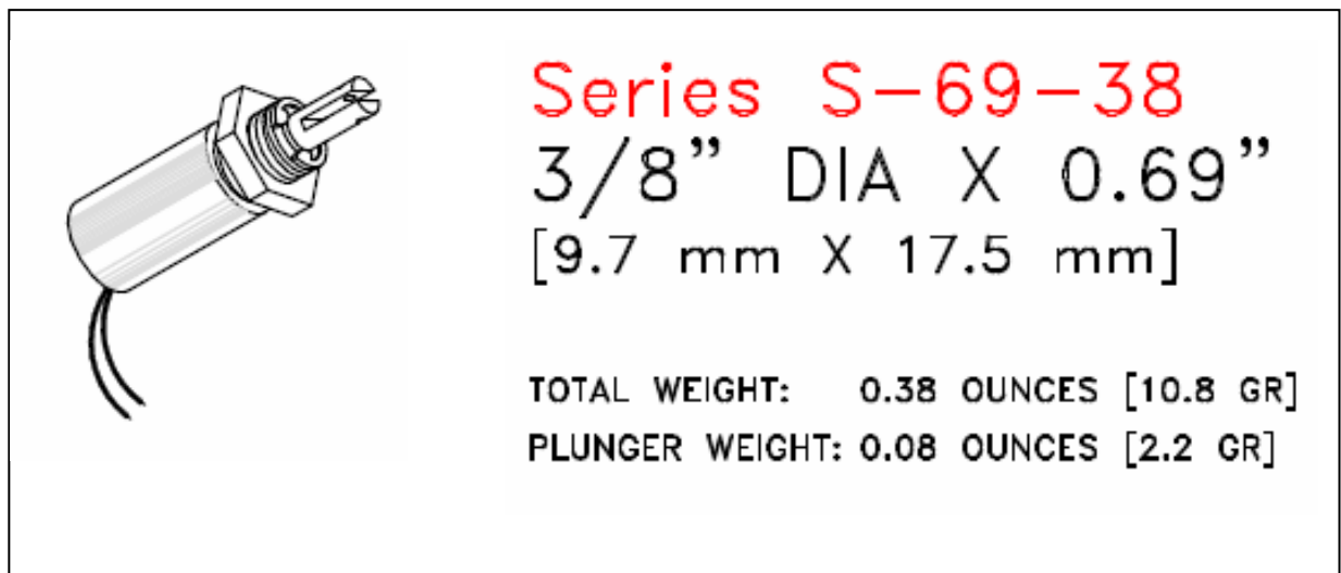
Figure 2. Tubular solenoid.
