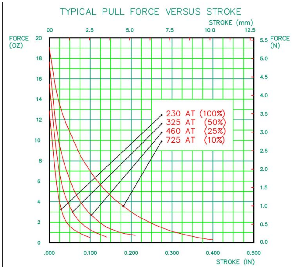
Figure 3. Solenoid pull force vs. stroke.
