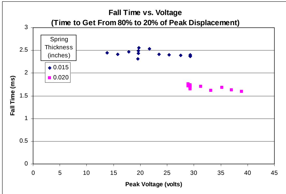
Figure 8. Fall time vs. voltage.
