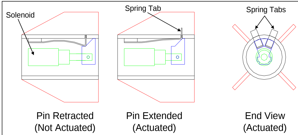
Figure 1. Actuator design concept.
