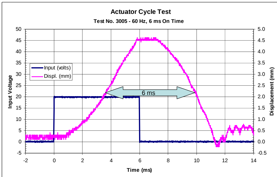
Figure 10. Single 20 V, 6 ms pulse, 0.015 in. spring.
