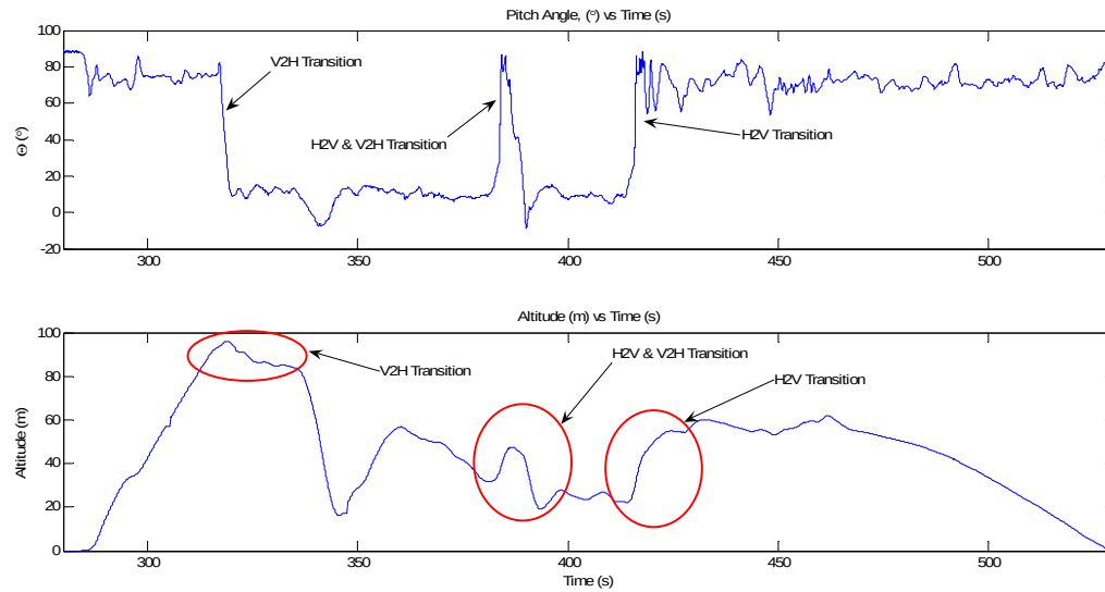
Figure 15: Altitude and Pitch Angle during 30/August Flight (2 Transitions each way). Altitude loss during the first Horizontal to Vertical (H2V) transition is ~5m; Altitude gain during the last Vertical to Horizontal (V2H) transition is ~40m.
