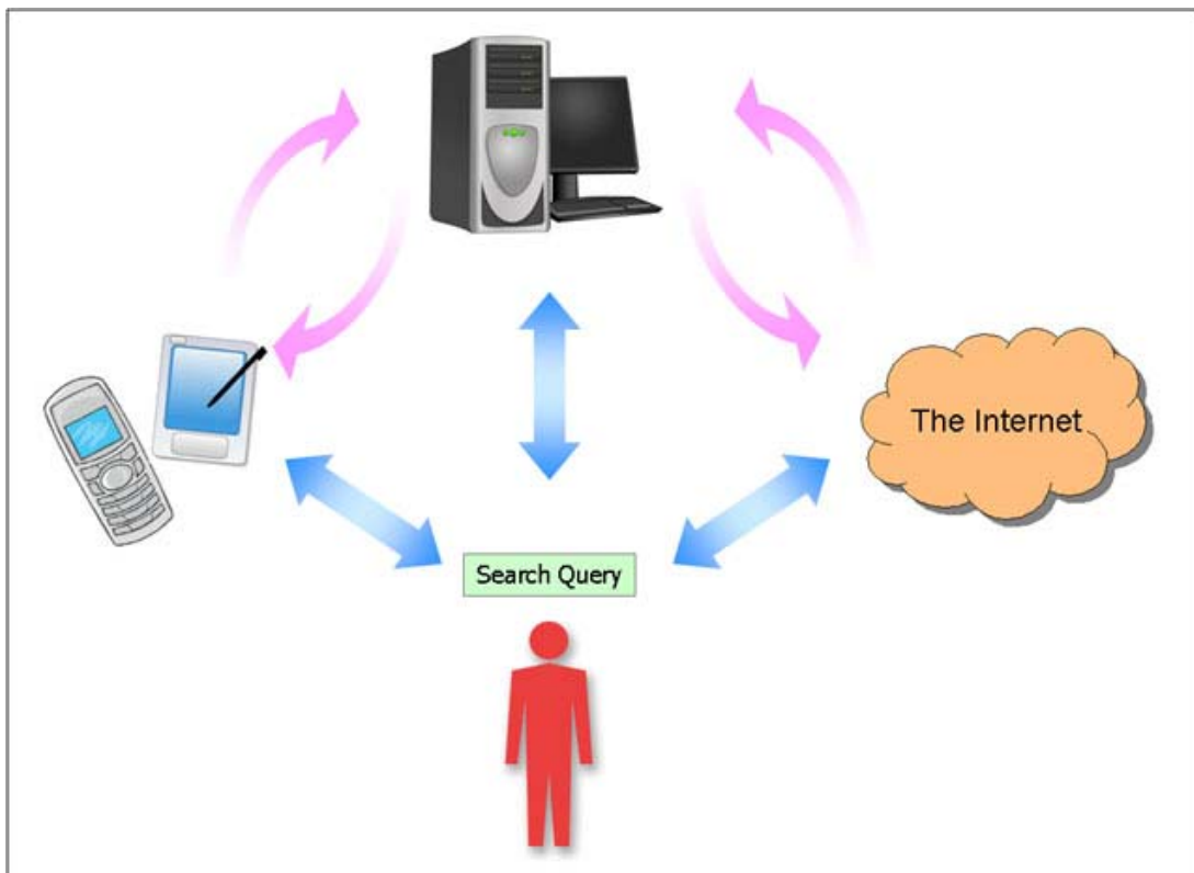
Figure 2. General Architecture.
