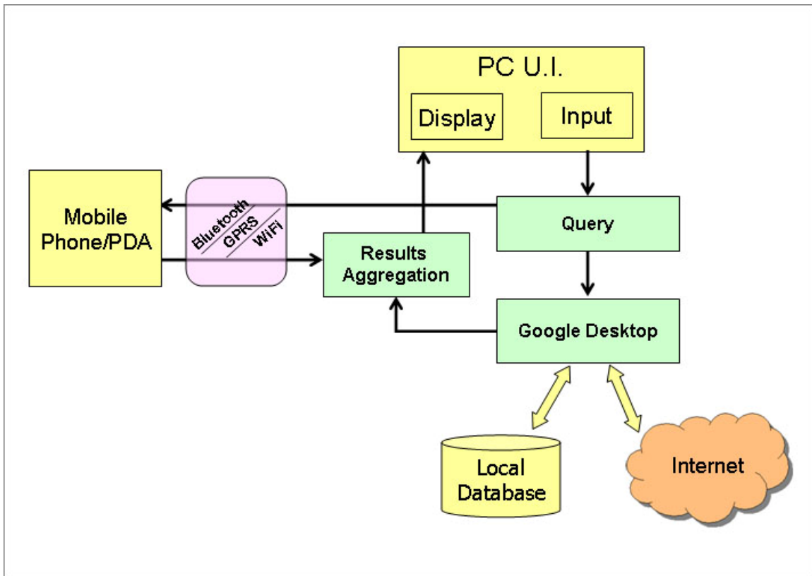
Figure 5. Component-Level Diagram.
