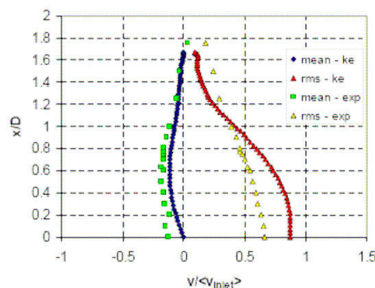
Figure 4-4 Experimental and URANS Simulation Data for Re = 55,000 and z/D = 2.0
