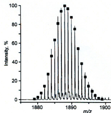
Fig. 4 MALDI-TOF mass spectrum for deuterated dimer d -1a. The simulated spectrum is represented by the black squares, and was calculated allowing for deuteration of 93% at the β-pyrrole positions and 33% at the aryl substituents.
