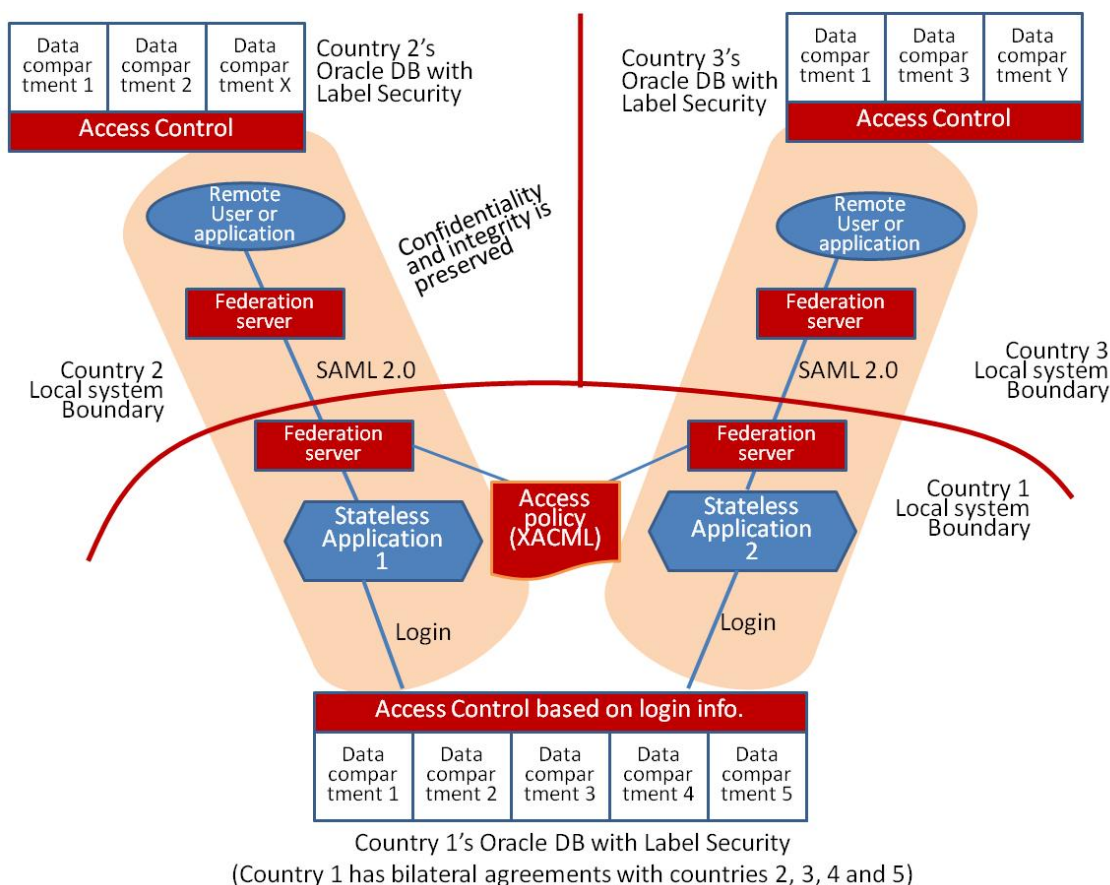
Figure 1- Simplified Architecture of the Proposed Solution for Bilaterally Sensitive Information on a Restricted Multilateral Network Environment
