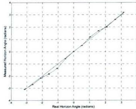
Measured horizon line roll angle vs. actual horizon roll angle. Error bars represent one standard deviation from 25 measurements.
