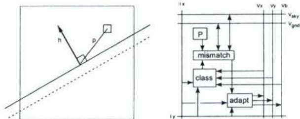
Left: The sign of the dot-product of a horizon vector ( h ) and the pixel vector ( p ) plus a bias determines the horizon line. The dotted line represents the horizon line with a positive bias. Right: Block diagram of processing in a single pixel. v_x , v_y , and v_b represent the horizon vector and each pixel's coordinate ( x, y ) is determined by i_x and i_y .
