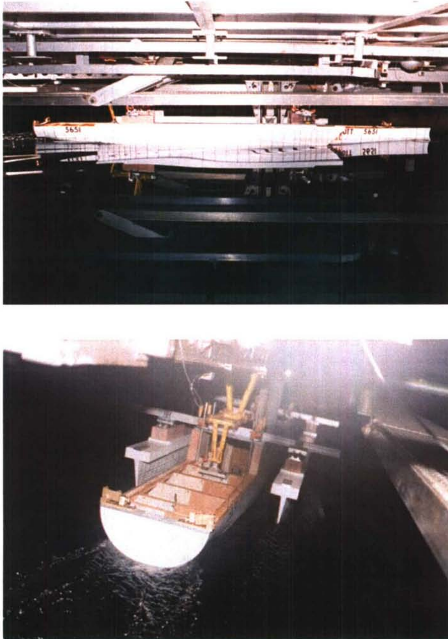
Figure 5. Photographs of Model 5651, representing HALSS at 11.5 m draft with various side hull configurations.
