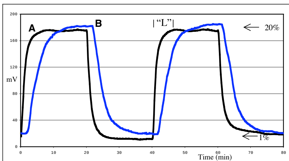
Figure 3. Oxygen Electrode Readings. Trace A, electrode only. Trace B, electrode and tissue culture dish
