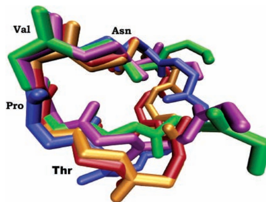
Figure 1. Overlay of the cyclic-[EKTPVNPGN] (red), cyclic-[EKTPVNPGQ] (blue), cyclic-[EMTPVNPGQ] (orange), and the EMTPVNPG (green) and EMTPVTNPG (purple) peptides from REMD simulations. Each structure represents the \beta -turn motif sampled during the dynamics.
