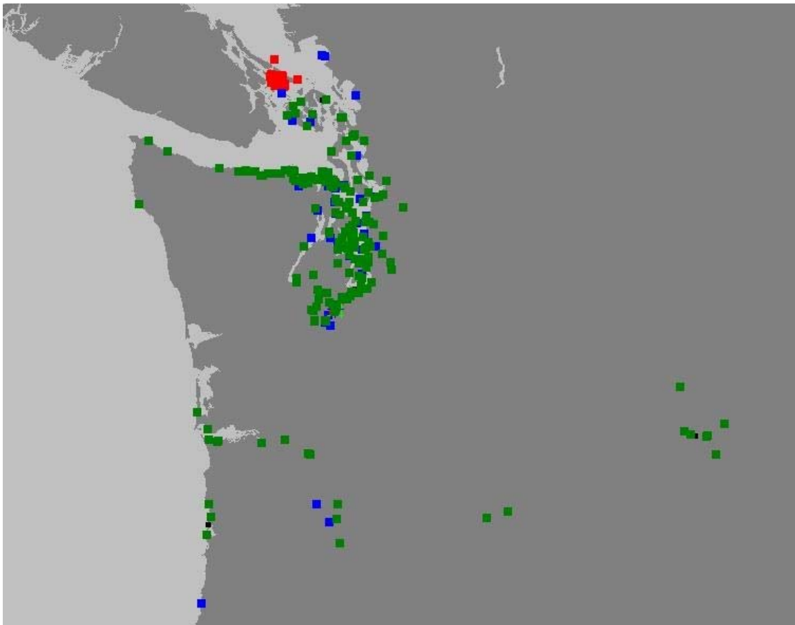
Figure 1. CAN Scatterplot
