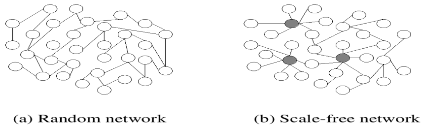
Figure 3. Network Types.
